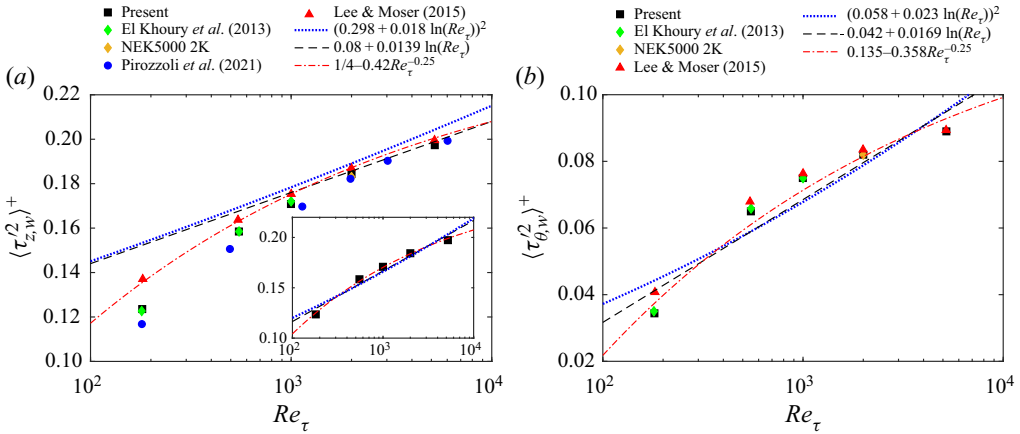
Figure 4. (a) Axial ( \langle \tau_{z,w}^2 \rangle^+ ) and (b) azimuthal ( \langle \tau_{\theta,w}^2 \rangle^+ ) wall shear stress fluctuations as a function of Re_\tau . The dotted, dashed and dashed-dotted lines in the inset of (a) denote \langle \tau_{z,w}^2 \rangle^+ = (0.225 + 0.0264 \ln(Re_\tau))^2 , \langle \tau_{z,w}^2 \rangle^+ = 0.016 + 0.0218 \ln(Re_\tau) and \langle \tau_{z,w}^2 \rangle^+ = 0.255 - 0.477 Re_\tau^{-1/4} , respectively.
