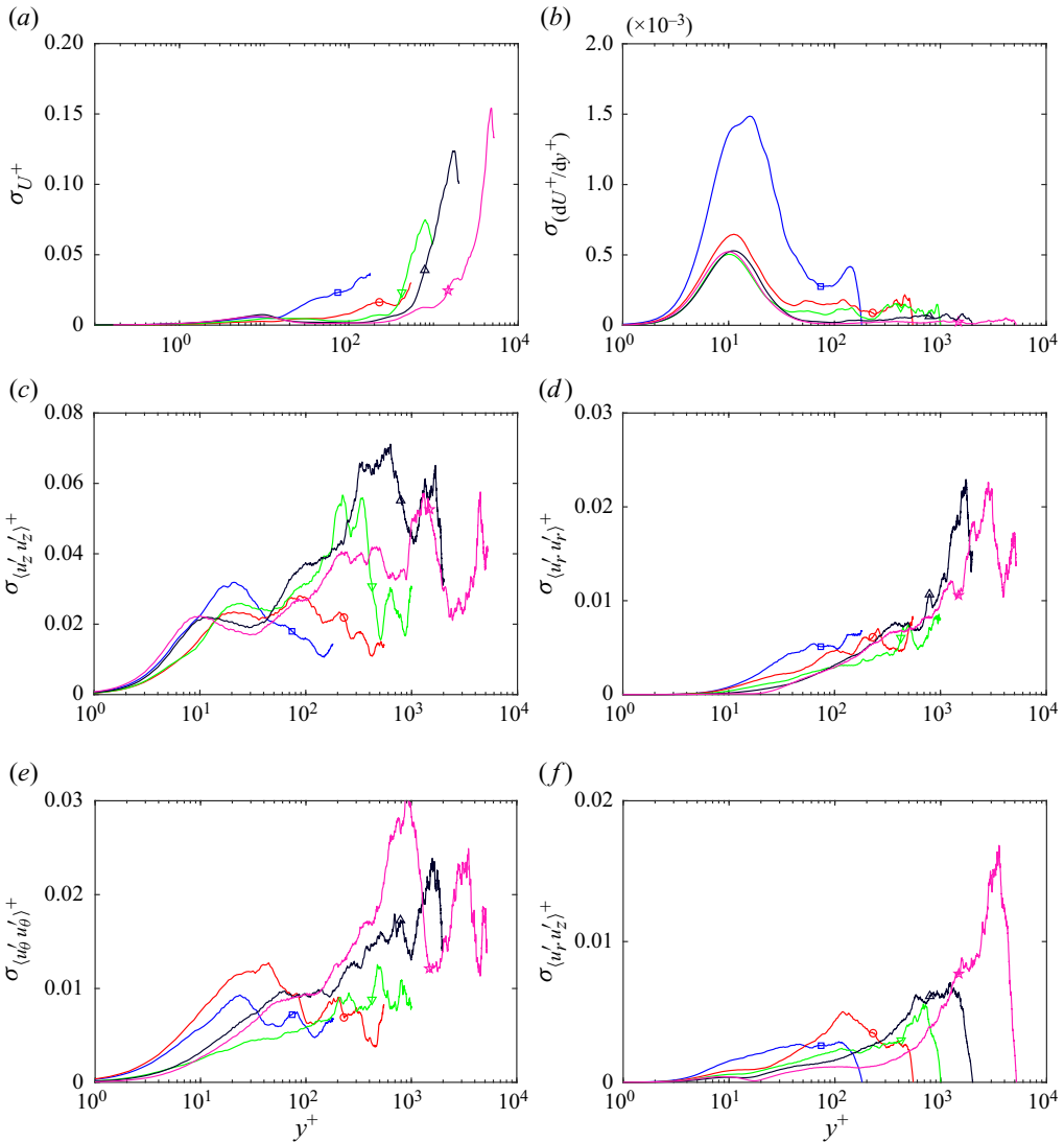
Figure 17. Estimated standard deviation of different statistical quantities: (a) U^+ , (b) \partial U^+/\partial y^+ , (c) \langle u_z^2 \rangle^+ , (d) \langle u_r^2 \rangle^+ , (e) \langle u_\theta^2 \rangle^+ , (f) \langle u_r u_z \rangle^+ .
