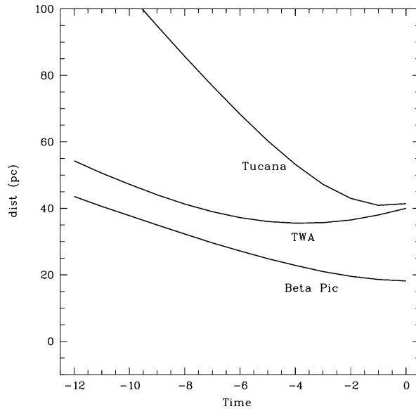
Figure 2. Distances between TWA22AB and three moving groups (TWA, \beta Pic and Tuc–Hor) for the past 12 Myr.
