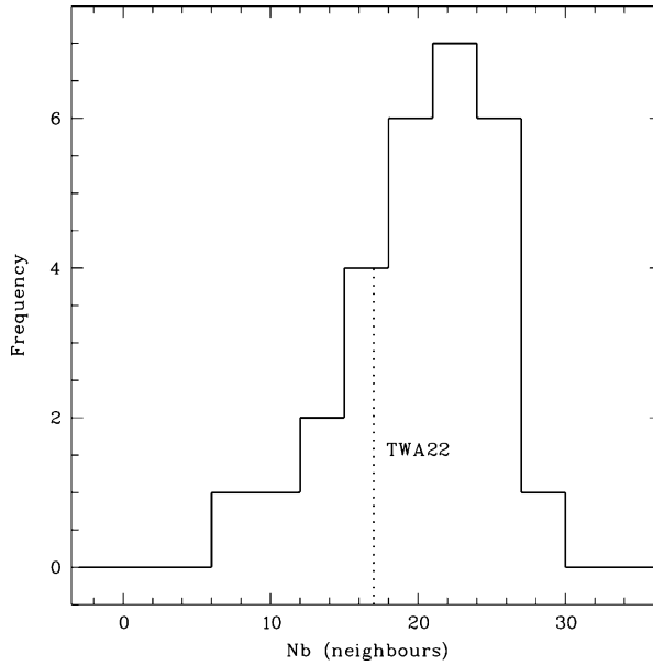
Figure 1. Number of \beta Pic members in a sphere of 2\sigma radius in the UVW space around each member. ( \sigma : velocity dispersion for this association.)
