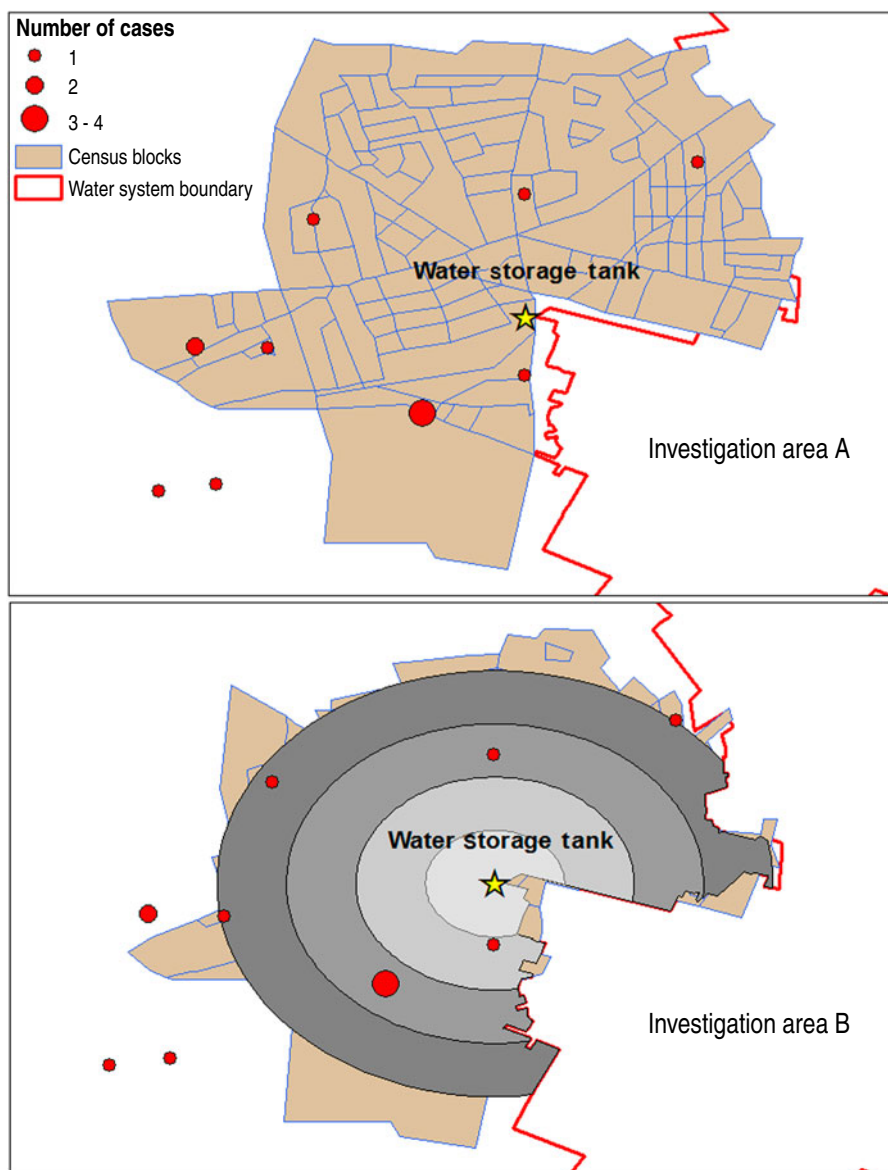
Fig. 1. Estimate of census blocks within an estimated area of influence of a water storage tank estimated by two independent methods, with overlay of case counts, 2003–2007. (a) Investigation area A; (b) investigation area B.
