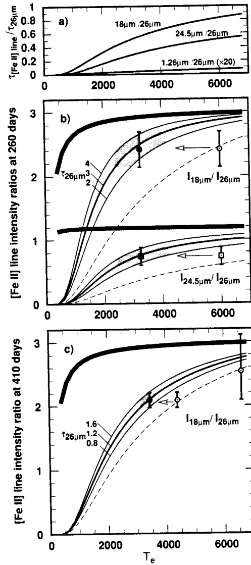
FIGURE 1. a.– \tau vs T_e ; b&c.– [Fe II] line intensity ratios vs T_e and \tau_{26 \mu\text{m}} .
