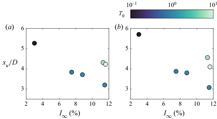
Figure 15. Location of the change of sign x_k/D in the spatial mean of D\kappa/Dt as a function of the free stream turbulence intensity I_\infty (horizontal axis) and integral time scale T_0 (colour axis), shown for (a) \lambda = 3.8 and (b) \lambda = 4.7 .
