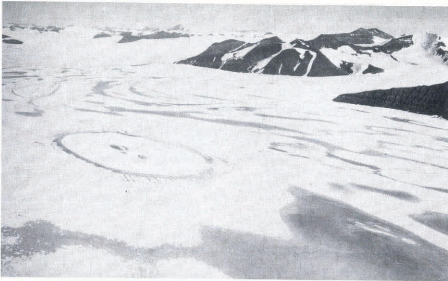
Fig. 2. The large ice doline (also called the ice caldera) on George VI Sound, Antarctica, taken from the air in January 1967. The doline is about 1.5 km in diameter. Uranus Glacier at top left and Eros Glacier from the upper right are shown entering the ice shelf. The dark streaks are meltwater lakes. Notice the similarity in shape to the ice blister in Figure 1 but the great difference in size. (Photograph by courtesy of C. W. M. Swithinbank.)
