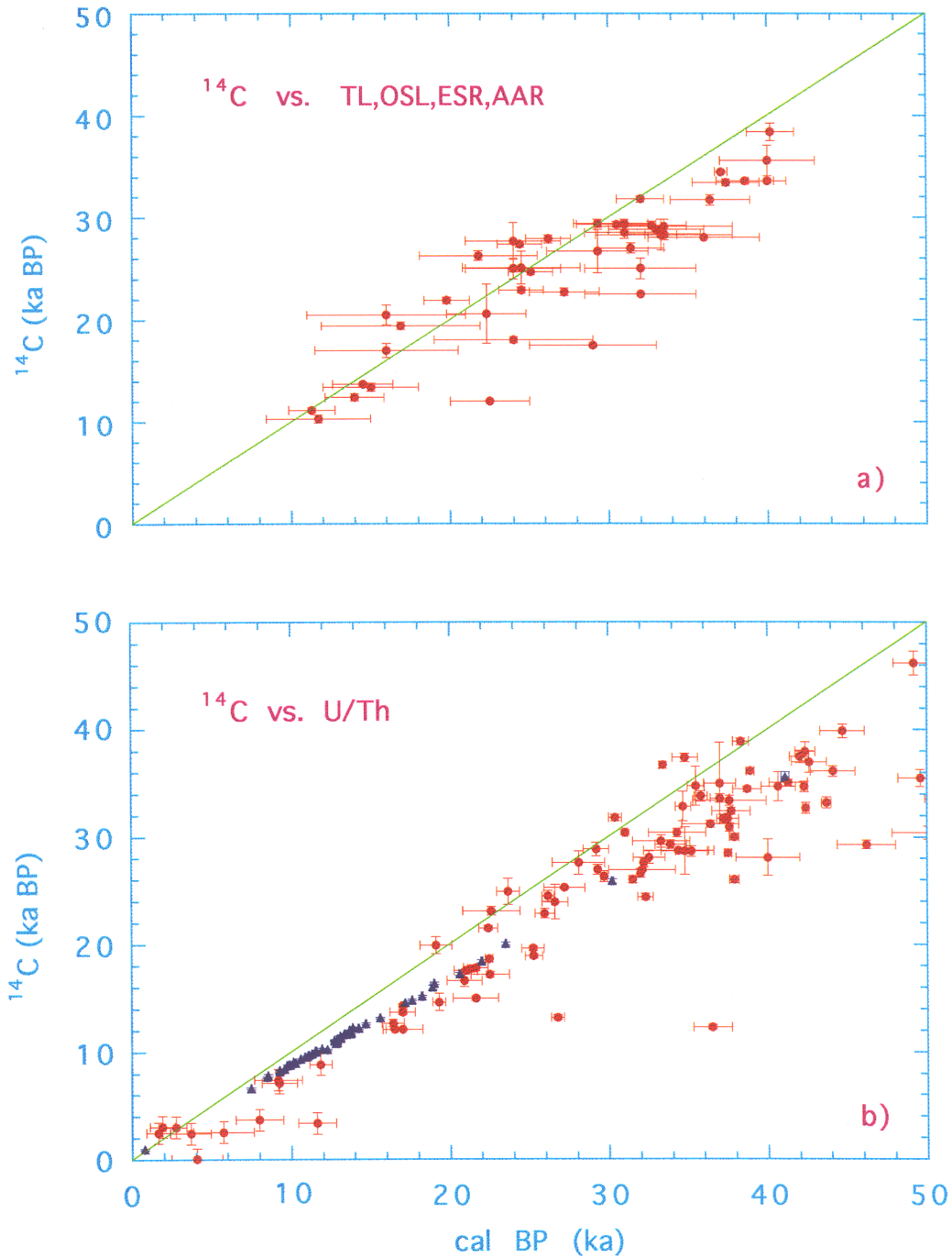
Figure 1 Compilation: comparison of 14 C versus other dating methods. a: TL, OSL, ESR, and AAR. b: U/Th dating.
