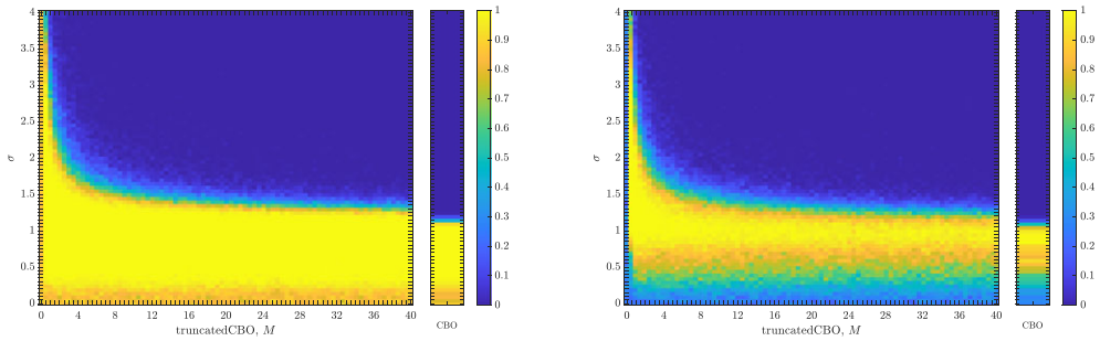
(a) Phase diagram of success probabilities of isotropic CBO with and without truncated noise at the example of the Ackley function f(v) = -20 \exp(-0.2/\sqrt{d} \|v\|_2) - \exp(1/d \sum_{k=1}^d \cos(2\pi v_k)) with d = 4 (b) Phase diagram of success probabilities of isotropic CBO with and without truncated noise at the example of the Rastrigin function f(v) = \sum_{k=1}^d v_k^2 + 2.5(1 - \cos(2\pi v_k)) with d = 4
