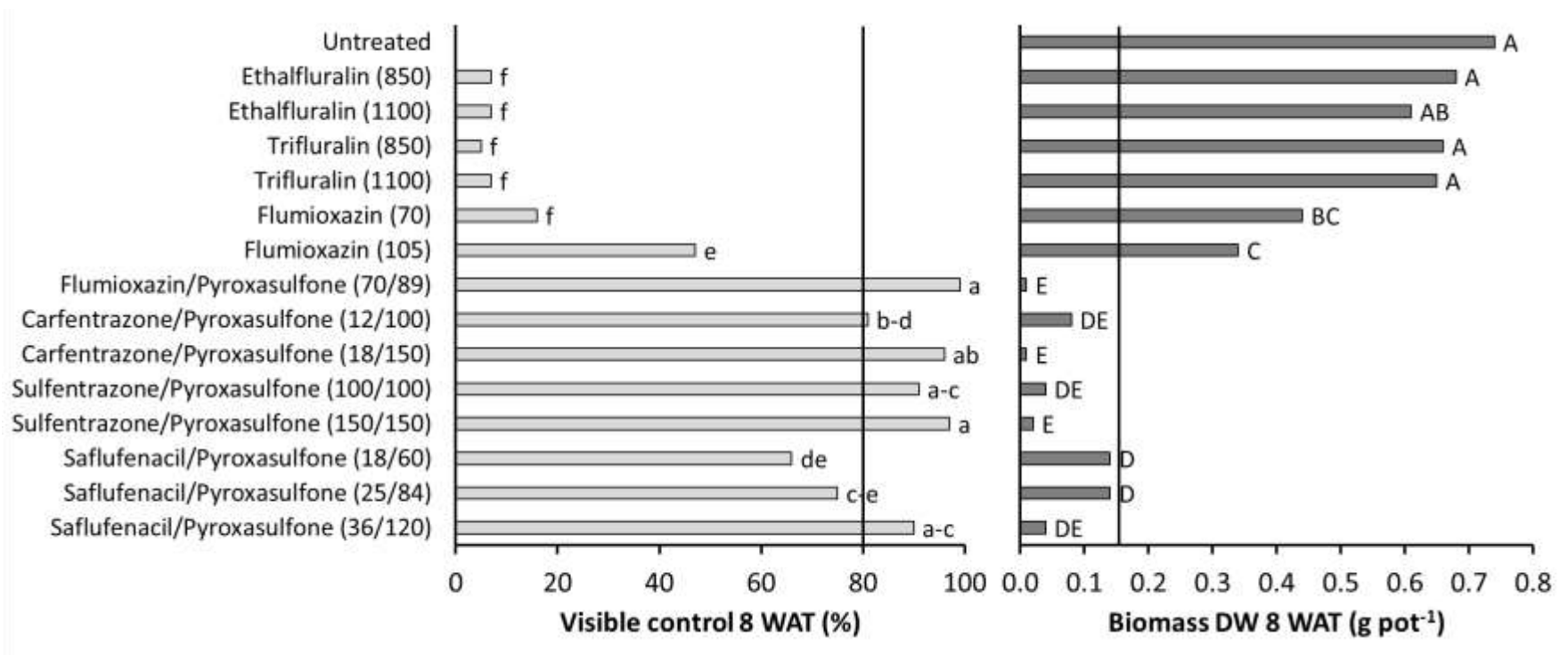
Figure 1. Visible control ( P < 0.0001 ) and biomass dry weight (DW; P < 0.0001 ) of downy brome 8 wk after treatment (WAT) with a range of preemergence soil-applied herbicides in combined analyses among sandy loam and clay loam soils and glyphosate-resistant and glyphosate-susceptible downy brome populations. Numbers in parentheses indicate the amount of each active ingredient in \text{g ai ha}^{-1} . Within subfigures, different letters indicate significant differences based on Tukey's honestly significant difference test ( \alpha = 0.05 ). Vertical lines indicate the threshold for 80% visible control or 80% reduction in biomass DW relative to the untreated control.
