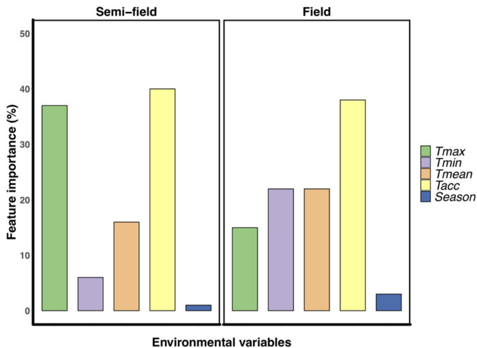
Figure 2. Feature importance analysis using Random Forest regressions examining the effect of environmental descriptor variables on the relative recapture rate (recapture ratio) of Ceratitis capitata following mark-release-recapture in either semi-field (panel A) or field (panel B). Environmental descriptors are; Tmean, mean recorded temperature during recapture period; Tacc, adult acclimation treatment experienced prior to release (thermal history); Season, time of year (i.e. summer or winter) when the release was conducted.
