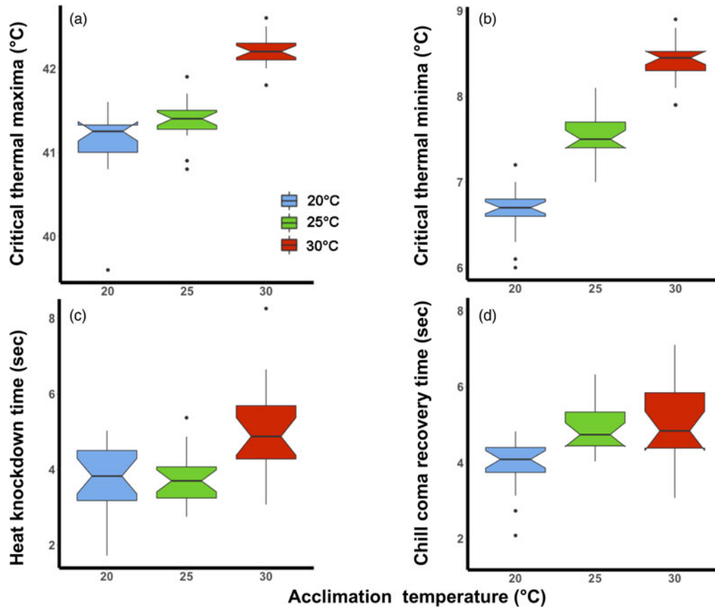
Figure 1. Laboratory thermal tolerance estimates of Ceratitidis capitata following acclimation to three environmental temperatures (20, 25, or 30°C) at the adult life stage; (a) critical thermal maxima, (b) critical thermal minima, (c) heat knockdown time and (d) chill coma recovery time. The box plots are coloured according to acclimation treatment, blue (20°C), green (25°C) and red (30°C). The notch on the boxplot illustrates the 95% confidence interval.
