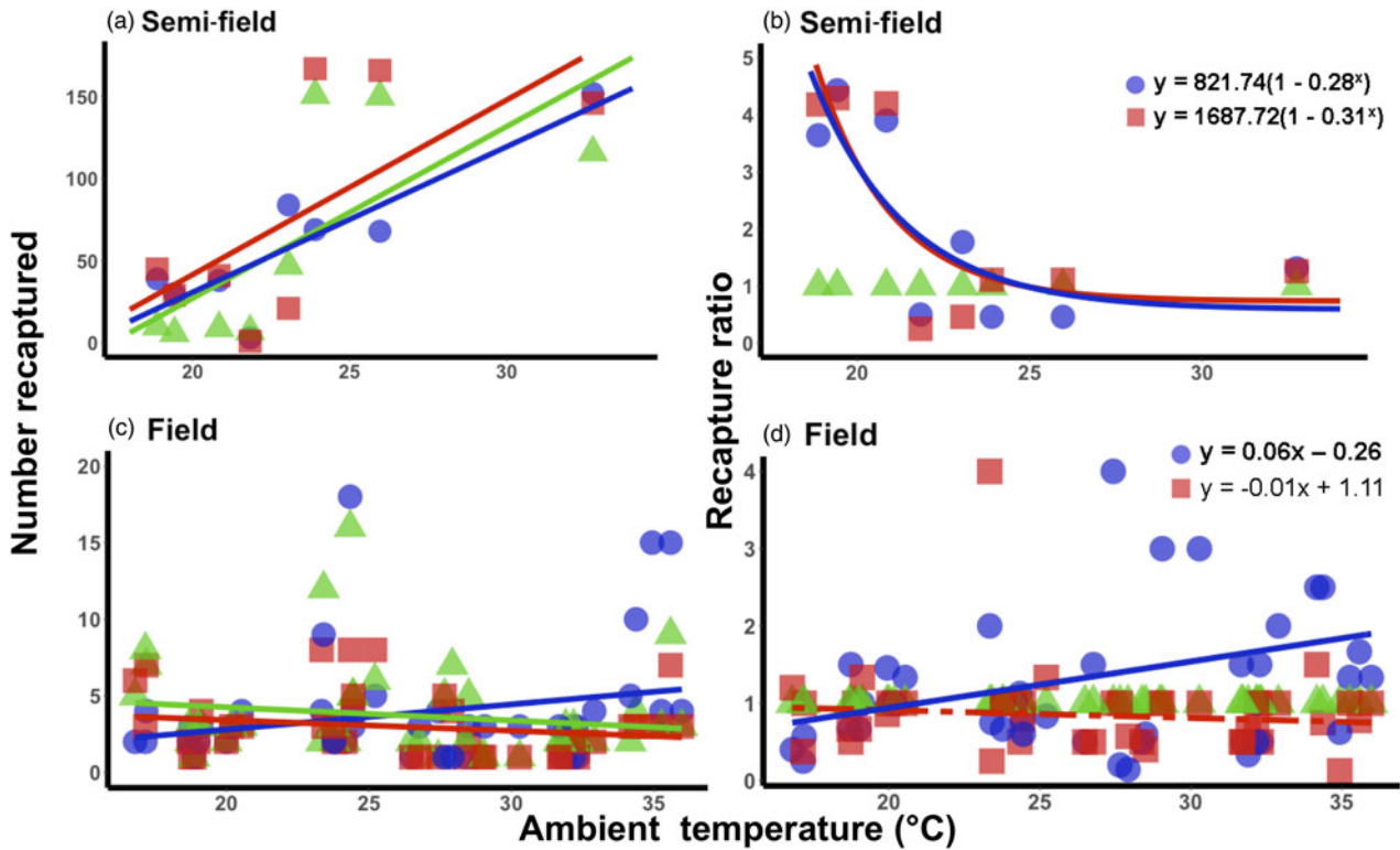
Figure 3. Relationship between mean ambient temperatures recorded during recapture period and the recapture ratio of Ceratitis capitata following mark-release-recapture after acclimation for semi- (a, b) and field (c, d) conditions, respectively. Data were transformed to \log(n + 1) in order to account for zero recapture, and recapture ratios determined relative to the 25°C control group. Each acclimation group's data were fitted separately (i.e. 20 and 30°C), with solid lines indicating significant responses and dashed, non-significant. Fitted model equations for the recapture ratio treatment groups (b, d) with bold values are indicative of significant effects.
