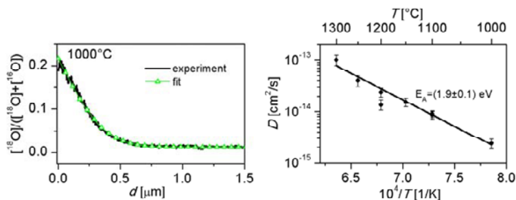
Fig. 1: ^{18}\text{O} diffusion profile in CTGS annealed in an ^{18}\text{O}_2 atmosphere for 48 hours at 1000 ^\circ\text{C} and corresponding fit as a function of reciprocal temperature. (see text for details).
