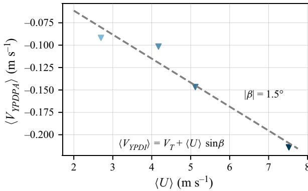
Figure 17. Here \langle V_{YPDI} \rangle against \langle U \rangle for the different incoming velocities with olive oil droplets measurements. A linear fit of the data is shown in dashed line.
