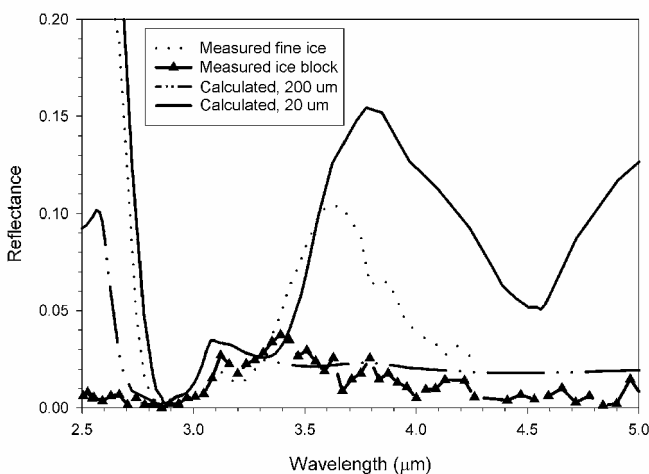
Fig. 1. Measured and calculated water ice at various grain-sizes. Measured frost and ice from Roush and others (1990). Calculations performed using the optical constants of Warren (1984) and the bidirectional radiative transfer model of Hapke (1981).
