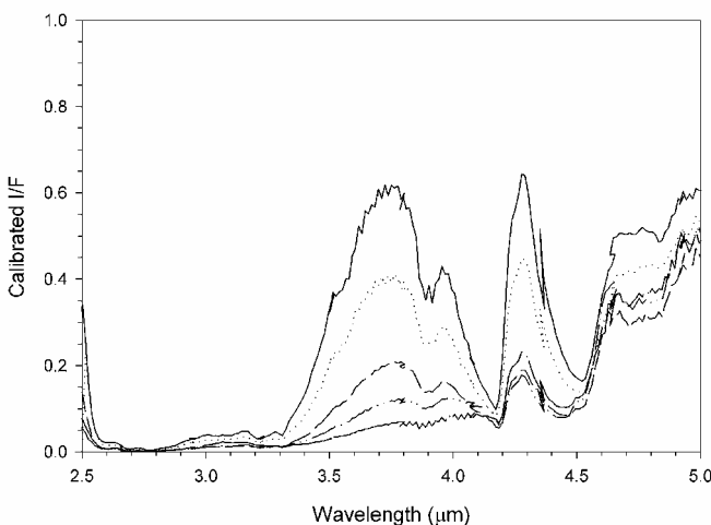
Fig. 8. Spectra corrected for viewing geometry and thermal emission. Note that the thermal contribution ( > 4.5\text{ }\mu\text{m} ) has been mostly equalized, while substantial variation in the 3.7\text{ }\mu\text{m} ice peak strength remains. Accurate correction for the \text{CO}_2 gas absorption (inverted peak between 4.2 and 4.5\text{ }\mu\text{m} ) was not attempted. Ice peak heights span the range of colors shown in Figure 6. Purple/black corresponds to the lowest peak in this figure, red the highest, with approximate color thresholds as indicated in Figure 6 caption.
