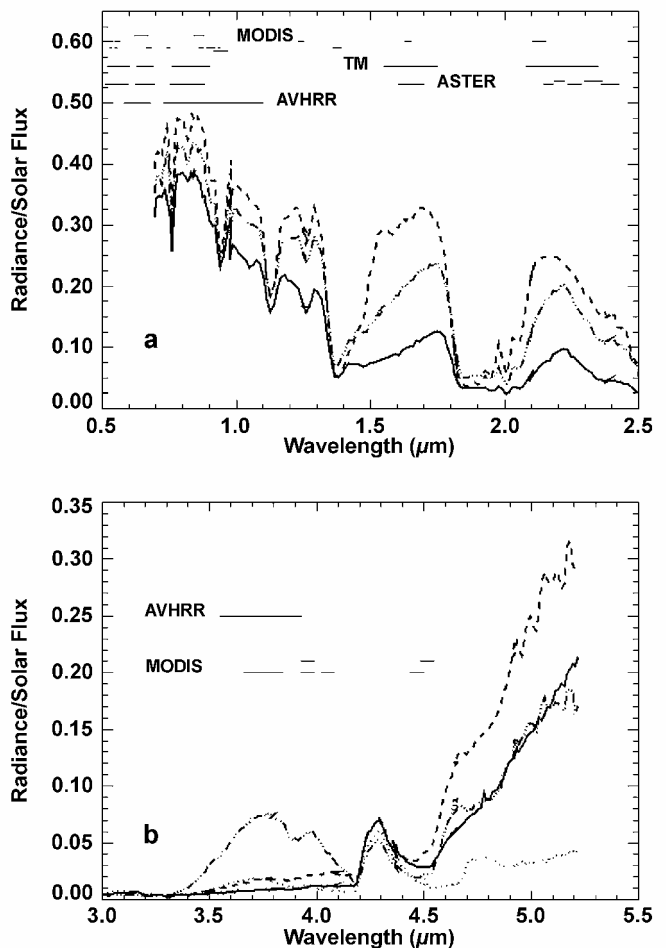
Fig. 4. Spectral variation within the NIMS data cube, 0.7– 2.5 \mu\text{m} (a) and 3– 5.5 \mu\text{m} (b). Spectra of individual pixels clearly show variations between normal atmospheric transmission (short dash in (a); solid in (b)) and increasing ice contributions as snow or ice cloud (dot-dash and solid in (a); dot-dash in (b)). Varying thermal emission is also evident in the strength of the radiance upturn beyond 4 \mu\text{m} (b). Band-passes for AVHRR, ASTER and MODIS are plotted for comparison.
