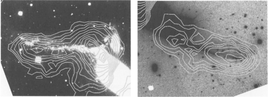
Figure 1. HI \lambda 21 cm contour map on a blue-band VLT image. The contour levels range from 0.2 to 1.2 \text{ Jy beam}^{-1} \text{ km s}^{-1} by steps of 0.1 . The HI peaks at the tip of the spiral arms coincide with regions of enhanced star formation.
