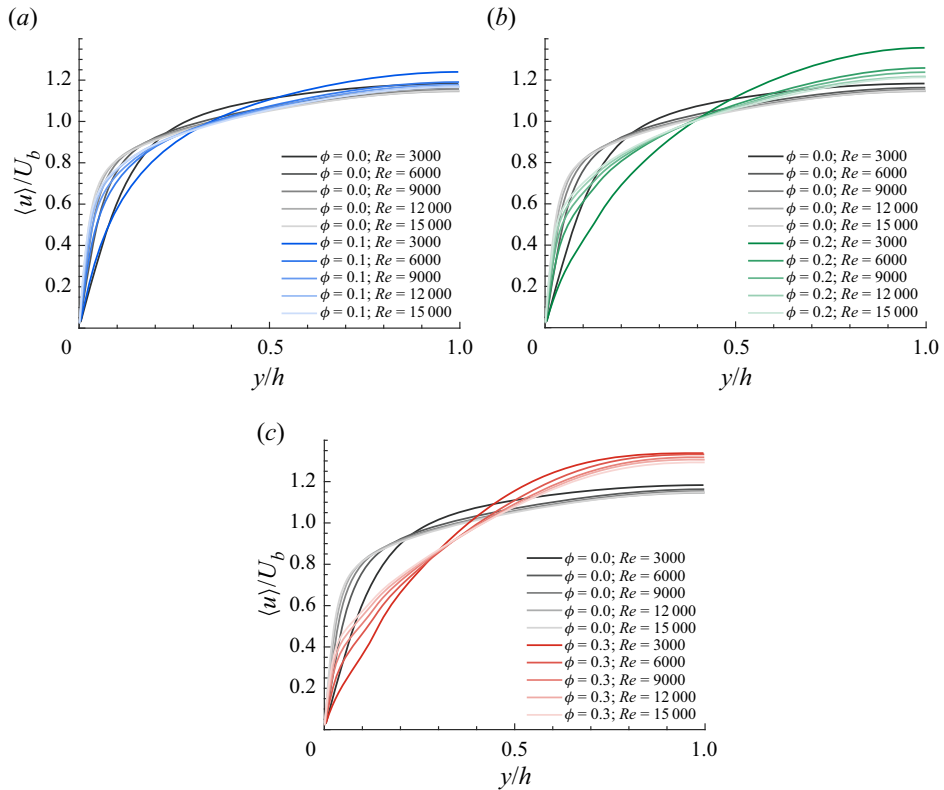
Figure 2. Outer-scaled mean fluid velocity profiles, compared with the single-phase data, for (a) \phi = 0.1 , (b) \phi = 0.2 and (c) \phi = 0.3 .
