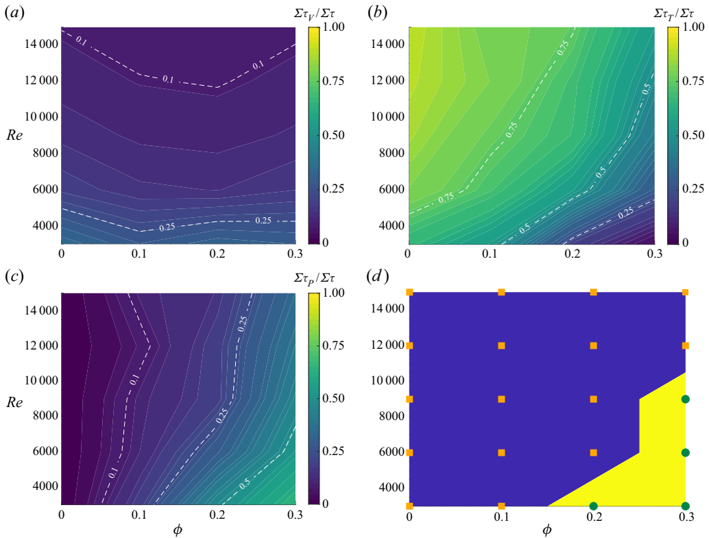
Figure 6. Contour map of the contribution of (a) viscous stress \Sigma\tau_V , (b) Reynolds stress \Sigma\tau_T and (c) particle-induced stress \Sigma\tau_P to the total momentum transport integrated across the channel; the white dashed lines denote iso-levels as guide for the eye. Panel (d) displays a map of the flow regimes in the Reynolds number–volume fraction plane, identified by the dominant contribution to the momentum budget. Blue colour: turbulent Reynolds stress dominated regime; yellow: particle stress dominated regime. The different symbols display the available simulation data.
