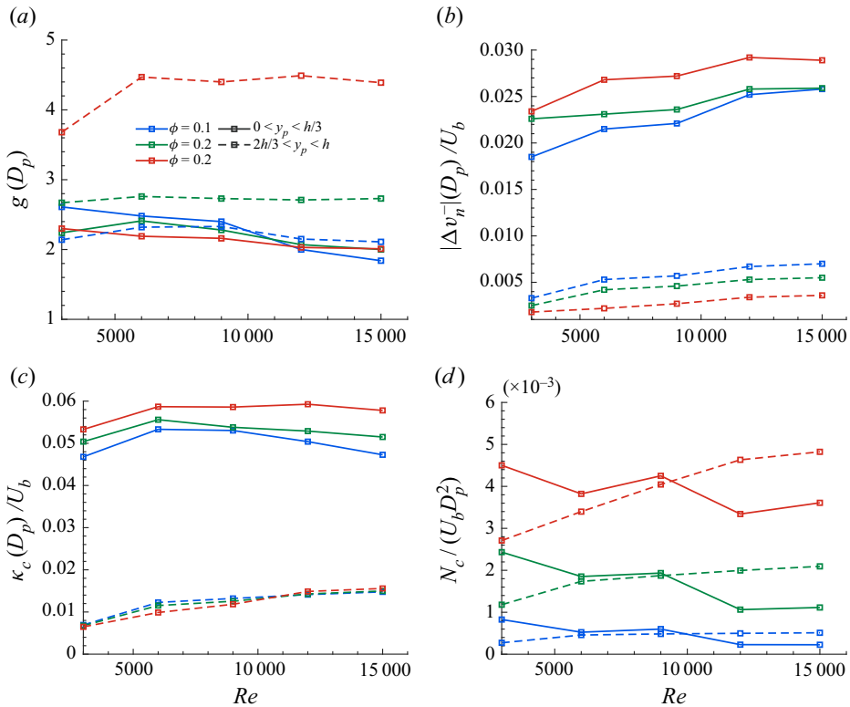
Figure 13. (a) The RDF, (b) magnitude of the relative approaching velocity and (c) collision kernel at contact ( r = D_p ), together with (d) collision frequency, N_c = \pi(\Phi)^2 D_p^2 \kappa_c(D_p) , vs the Reynolds number for different volume fractions. Solid lines denote averaging over particles located at 0 < y_p < h/3 and dashed lines 2h/3 < y_p < h .
