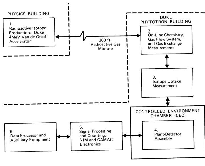
Fig 1. Outline of the integrated system for studying the carbon allocation in plants using radioactive tracers under controlled environment conditions
