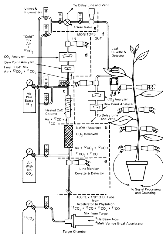
Fig 2. The experimental layout. a. Line Monitor. b. Removal of target material. c. Oxidation of ^{11}\text{CO} . d. In Line Monitor, \text{CO}_2 analyzer and dew point analyzer. e. Final In Monitor. f. ^{12}\text{CO}_2 Out Monitor, leaf cuvette, and plant and detector assembly in the controlled environment chamber (CEC).
