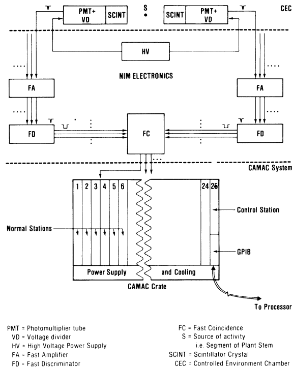
Fig 3. Signal processing and counting using NIM and CAMAC systems. NIM = Nuclear Instrumentation Electronic Modular CAMAC = Computer Automated Measurement and Control.
