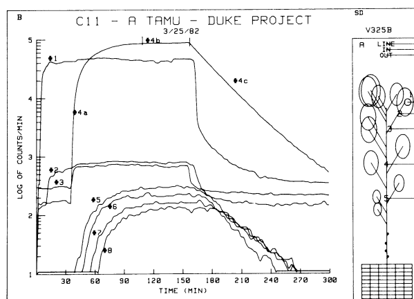
Fig 4. Live-time display of tracer profiles of Velvet Leaf ( Abutilon theophrastic Medic ). A. Plant geometry with detectors #1 monitoring the leaf and detector pairs #2, #3, #4, and #5 monitoring the phloem activity. B. Profile #1 shows the line activity as recorded by the Line Monitor, #2 and #3, the input and output activities as recorded by the Input and Output Monitors, respectively. Profile #4-a, #4-b, and #4-c show the time-dependent, the steady-state, and the washout behavior of the leaf, respectively. Profiles 5, 6, 7, and 8 show the tracer profiles in the phloem as monitored by detector pairs #2, #3, #4, and #5 (fig 4A).
