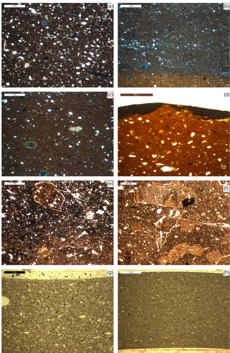
Fig 18. Sonari: photomicrographs of ceramic thin sections of samples. a) SNR 4 ; b) SNR 5 ; c) SNR 8 ; d) SNR 13 ; e) SNR 12 ; f) SNR 14 ; g) blue-on-white SNR 102 ; h) SNR 101 white porcelain samples. Photomicrographs a–c were taken in cross polarised light, and d–h in plane polarised light. Photographs: M Spataro.
