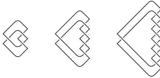
FIGURE 2. Front diagrams for the Legendrian (2, -(p - 1)/2) -torus knots with (tb, r) = (1 - p, (p - 5)/2) for p = 7, 11, 15 . (Since r depends on the orientation, the topmost strand in each front should be oriented from left to right.) Each of these fronts has an ungraded normal ruling with switches at every crossing.
