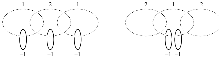
FIGURE 3. The minimal symplectic fillings W_{8,3}(1, 2, 1) (left) and W_{8,3}(2, 1, 2) (right) of (L(8, 3), \xi_{\text{can}}) . In each diagram the dotted curves give a surgery description of S^1 \times S^2 ; we identify this with \partial(S^1 \times D^3) by an orientation-preserving diffeomorphism and then attach 2-handles to S^1 \times D^3 along the solid curves in its boundary as indicated.
