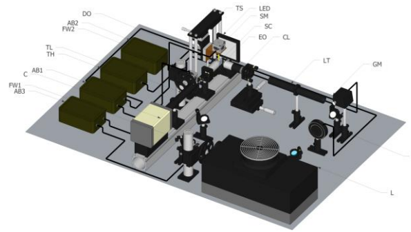
Figure 1. Schematic of the Light Sheet Fluorescence Microscope at IGC.
