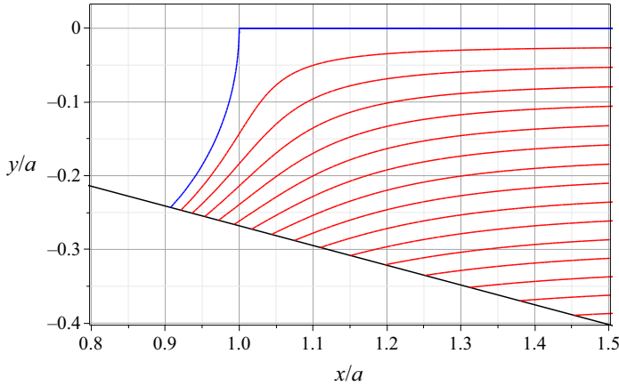
Figure 6. Pressure contours for beach angle \gamma = 15^\circ . Blue contour: free surface p = 0 . Contours: p/(\rho ga) = 0, [0.025], 0.375 ; maximum at lower right. Hydrostatic pressure is in the far field as x \rightarrow \infty .
