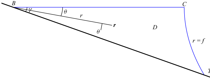
Figure 4. Sketch of fluid domain on a beach (black line); polar coordinates r, \theta centred at origin B , with unit vectors' directions indicated. Gravity g is vertically down. Free-surface sections are BC along the x -axis, and CT at the forward face. The shape, r = f(\theta) , of CT is found as part of the solution.
