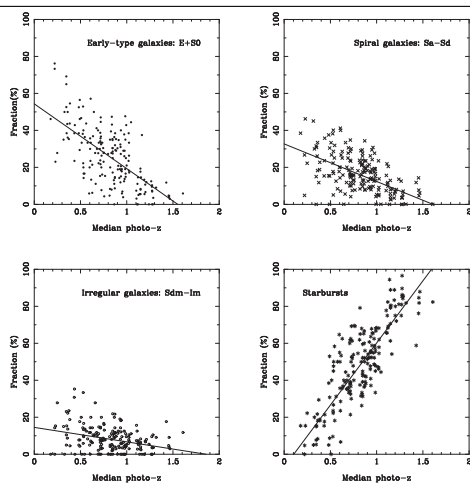
Figure 1. Fractions of four SED categories as the functions of redshift.
