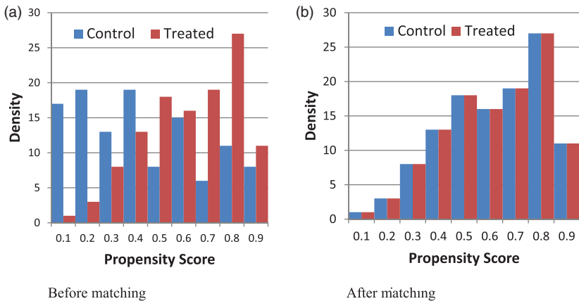
Figure 2. Regions of common support before (panel a) and after (panel b) nearest neighbor matching with replacement
