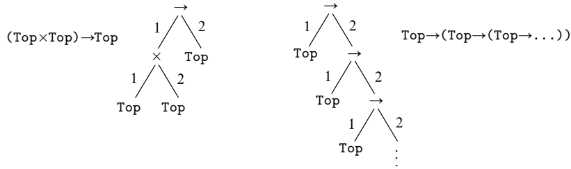
Fig. 2. Sample tree types.
