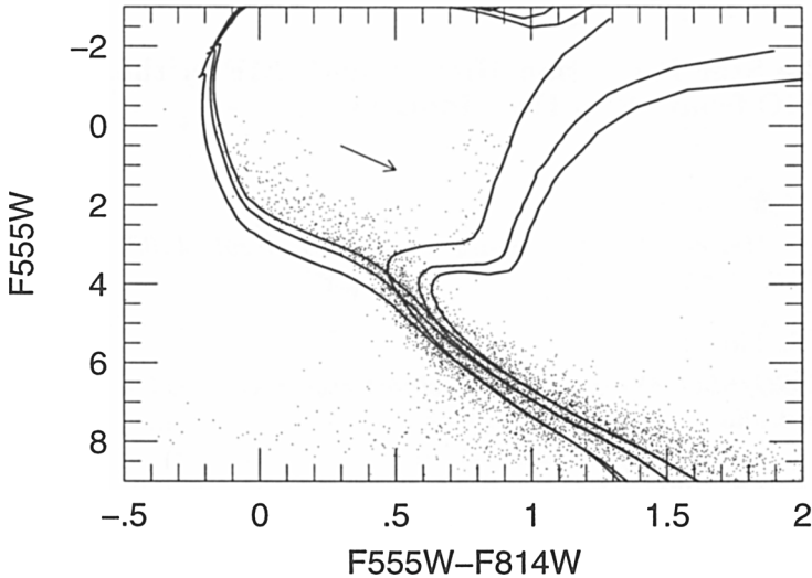
Figure 1. The color-magnitude diagram of one outer LMC field. Isochrones are for 1 and 10 Gyr with Z=0.0004 , 0.004 , and 0.008 .
