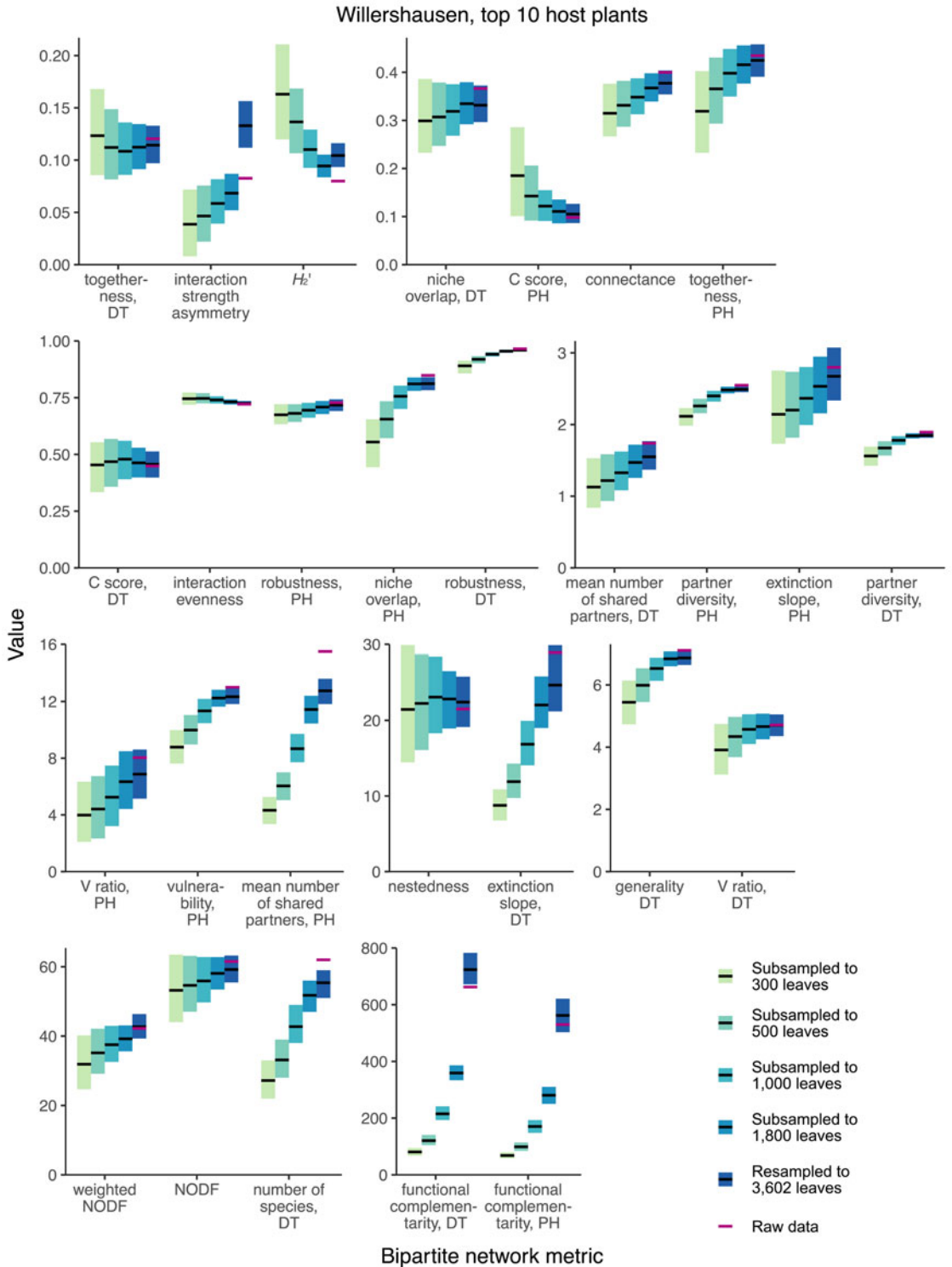
FIGURE 5. Mean values and 95% confidence intervals for bipartite network metrics generated by resampling and subsampling data for the 10 host plants at Willershausen represented by the highest numbers of leaves. DT, damage type; PH, plant host.
