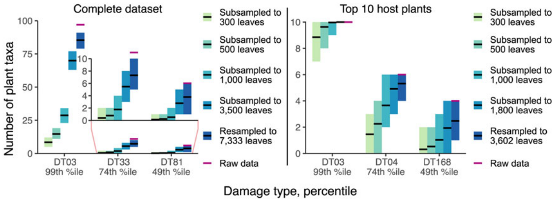
FIGURE 7. Mean values and 95% confidence intervals for the number of plant taxa on which various damage types appear, calculated with the Willershausen dataset.
