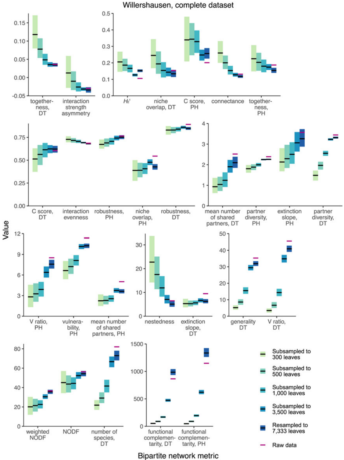
FIGURE 3. Mean values and 95% confidence intervals for bipartite network metrics generated by resampling and subsampling the cleaned Willershhausen dataset in its entirety. DT, damage type; PH, plant host.
