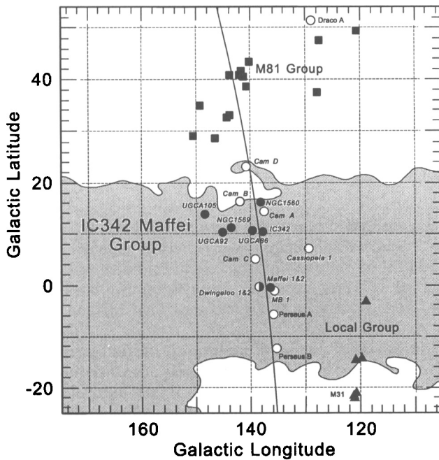
Figure 2. The distribution of galaxies in the area of the IC342/Maffei group (indicated by circles) along the supergalactic equator in galactic coordinates. Galaxies detected since 1994 are shown by open circles.
