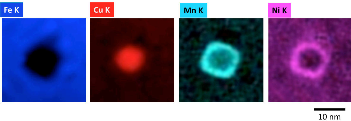
Figure 3: EELS multivariate statistical analysis reconstructed spectrum images corresponding to a thermally-aged precipitate nucleated at the matrix of low alloy steel weld aged for 49,800 hours.
