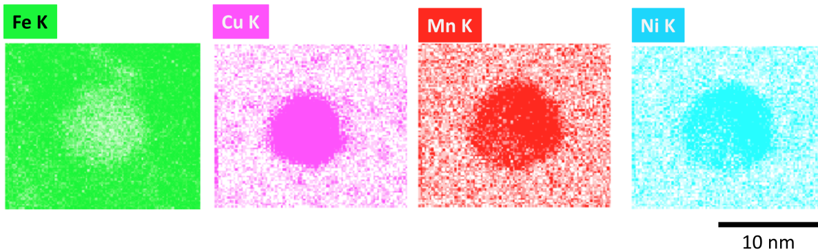
Figure 2: EDS spectrum images corresponding to a thermally-aged precipitate nucleated at the matrix of low alloy steel weld aged for 18,620 hours.
