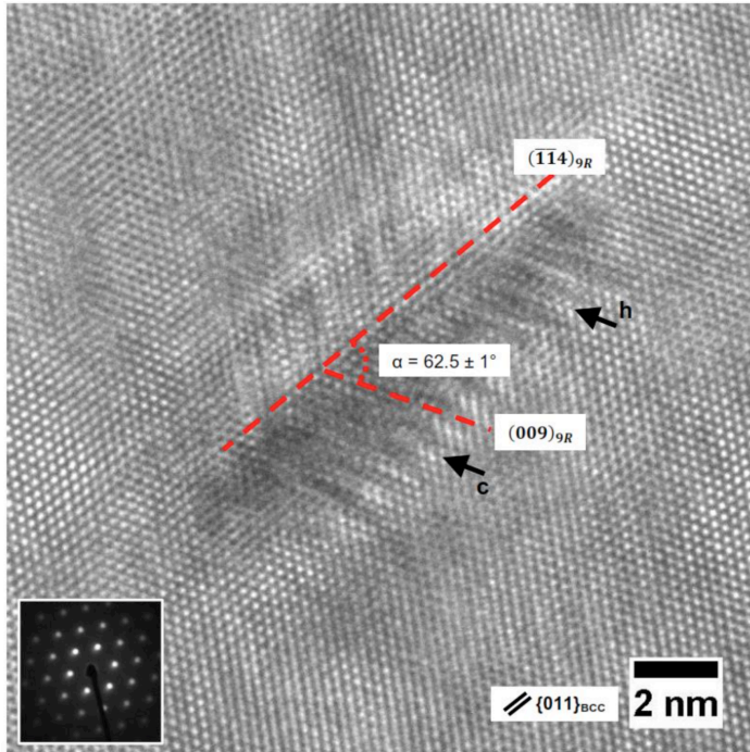
Figure 1: High resolution transmission electron image taken along \langle 111 \rangle_{Fe} showing a twinned 9R structure Cu precipitate (8 nm) in WV steel weld after thermal ageing for 49,800 hours at 365 °C. The angle \alpha between the (009)_{9R} basal and (\bar{1}\bar{1}4)_{9R} twin planes is 62.5 \pm 1^\circ . The 2-layer fringe spacing at the position of a hexagonal-type stacking faults is indicated. Similarly, the 4-layer fringe spacing at the position of a cubic-type stacking fault is also indicated.
