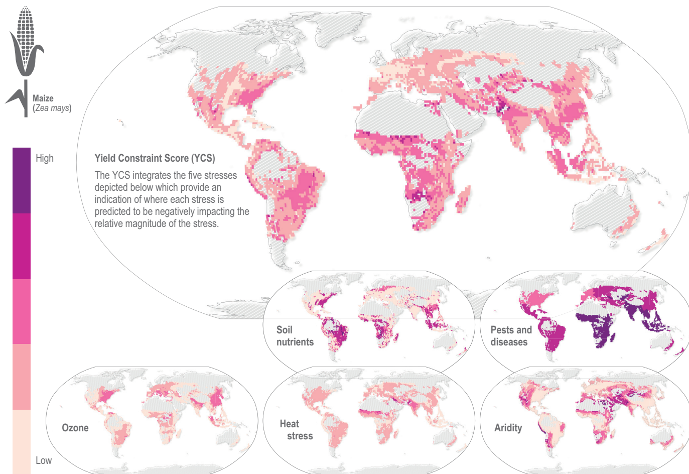
Figure AI.21 | Climatic and environmental stresses on global production of maize. Larger map depicts the combined effect of five stress on yield represented as a Yield Constraint Score (YCS) on a five-category scale from low stress to high stress (Mills et al., 2018). Higher temperatures enhance not only ozone production but also ozone uptake by plants, thus exacerbating yield loss and quality damage. Data are available at Sharps et al. (2020). All data are presented for the 1 × 1° (latitude and longitude) grid squares. [5.4.1; Figure 5.4]
