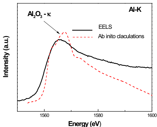
Figure 4. Experimental and calculated Al-K ionization edge sintered Al-C ( \text{Al}_2\text{O}_3 - \kappa )
