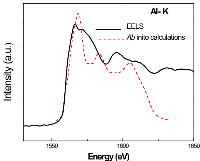
Figure 2. Experimental and calculated Al-K ionization edge of pure Al ( \text{Al}_2\text{O}_3 - \alpha )
