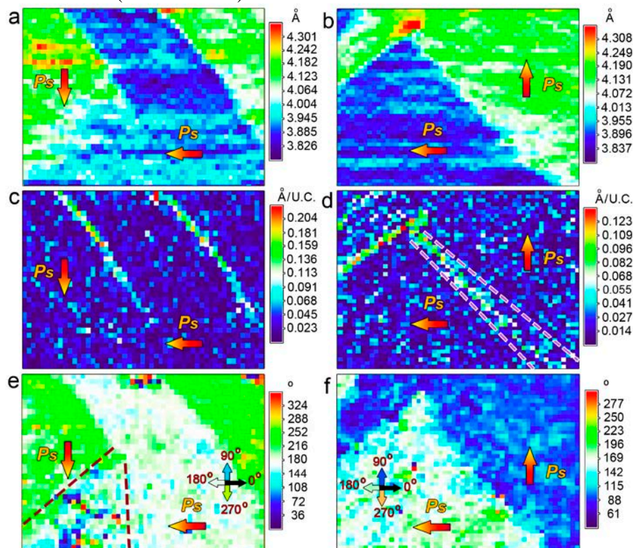
Figure 1. Two-Dimensional mappings of structural and electric behaviors showing the differences between 90^\circ CDWs and 90^\circ UCDWs. (a, b) Out-of-plane lattice spacing mapping for the 90^\circ PCDW and NCDW. (c, d) Lattice gradient mappings (lattice gradient of the out-of-plane lattice mappings along in-plane direction, mapped unit-cell by unit-cell) for the two types of domains. Note the alleviated lattice gradient across the 90^\circ CDWs, especially of the 90^\circ PCDW, compared with sharp lattice gradient across the 90^\circ UCDWs. (e, f) P_s angle mappings for the two types of domains. The definition of 0^\circ , 90^\circ , 180^\circ , and 270^\circ are marked with colored arrows with corresponding color-scale. In case of the 90^\circ PCDW, the P_s angles are markedly disordered.
