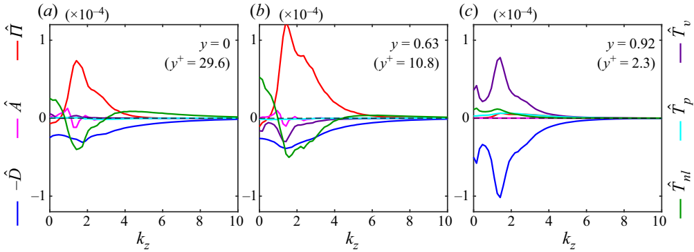
Figure 11. TKE spectral balance (5.3) at different y locations: (a) mid-plane, y = 0 ; (b) y = 0.63 ; (c) near-wall, y = 0.92 . Shown is a patterned case at Re = 400 .
