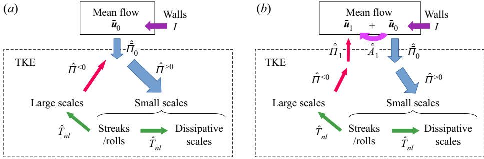
Figure 8. Illustration of the mean-flow–TKE interaction for (a) the uniformly turbulent state, and (b) the patterned state. In the uniform state, \hat{\Pi}_0 \simeq \hat{\Pi}^{<0} + \hat{\Pi}^{>0} , while in the patterned state, \hat{\Pi}_0 \simeq \hat{\Pi}^{>0} and \hat{\Pi}_1 \simeq \hat{\Pi}^{<0} .
