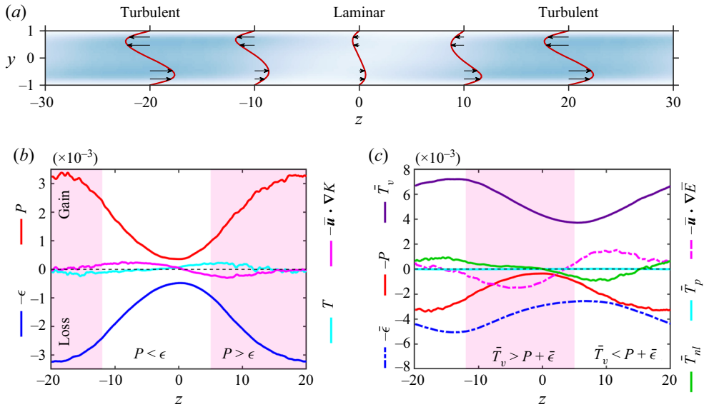
Figure 6. (a) Mean profiles of the deviation from laminar flow ( \bar{W} - W_b ) and the TKE (white 0, blue 0.08) in a turbulent–laminar pattern at Re = 400 centred around the laminar region at z = 0 . (b) TKE and (c) mean-flow energy budgets for Re = 400 . Each term is integrated over the upper half of the domain, y \in [0, 1] , where advection by the mean flow is towards the right. In (b), the regions where P > \epsilon are shaded. There is a transfer of turbulent energy from shaded to non-shaded regions. In (c), the regions where \bar{T}_v > P + \bar{\epsilon} are shaded. There is a transfer of mean-flow energy from shaded to non-shaded regions.
