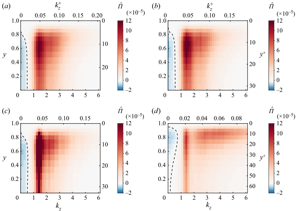
Figure 13. Visualisations of production \hat{\Pi}(y, k_z) for different Re and states. The cross-channel range is from the mid-plane ( y = 0, y^+ = Re_\tau , lower axis) to the wall ( y = 1, y^+ = 0 , upper axis). The dashed line separates positive from negative values for small k_z . (a) Pattern, Re = 400 ( Re_\tau = 29.7 ). (b) Pattern, Re = 430 ( Re_\tau = 31.9 ). (c) Uniform, Re = 430 ( Re_\tau = 33.0 ). (d) Uniform, Re = 1000 ( Re_\tau = 66.4 ).
