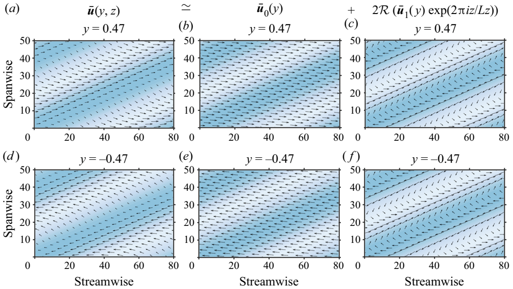
Figure 4. Mean-flow decomposition in two Fourier modes \bar{u}_0 and \bar{u}_1 (3.4), visualised in the planes y = \pm 0.47 at Re = 400 . Colours show TKE: turbulent and laminar zones are respectively in blue and white.
