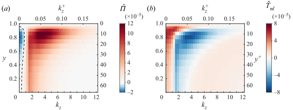
Figure 15. (a) Production and (b) nonlinear transfer spectra in a non-tilted domain with (L_{strm}, L_{span}) = (30, 20) for Re = 1000 ( Re_\tau = 66 ).
