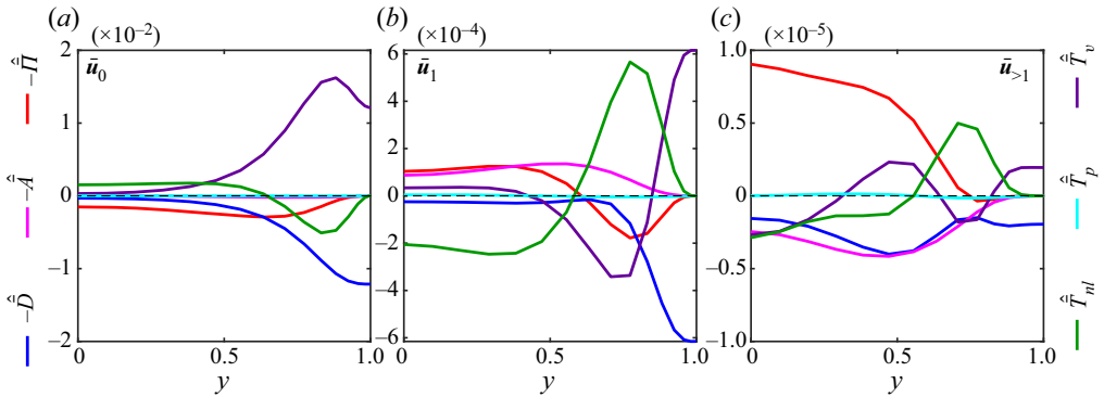
Figure 12. Evolution of the mean-flow energy balance (5.5) with y , for k_z = 0 , k_z = 2\pi/L_z , and summed over k_z > 2\pi/L_z . (Values for y < 0 are obtained by reflection in y = 0 .) Shown is a patterned case at Re = 400 .
