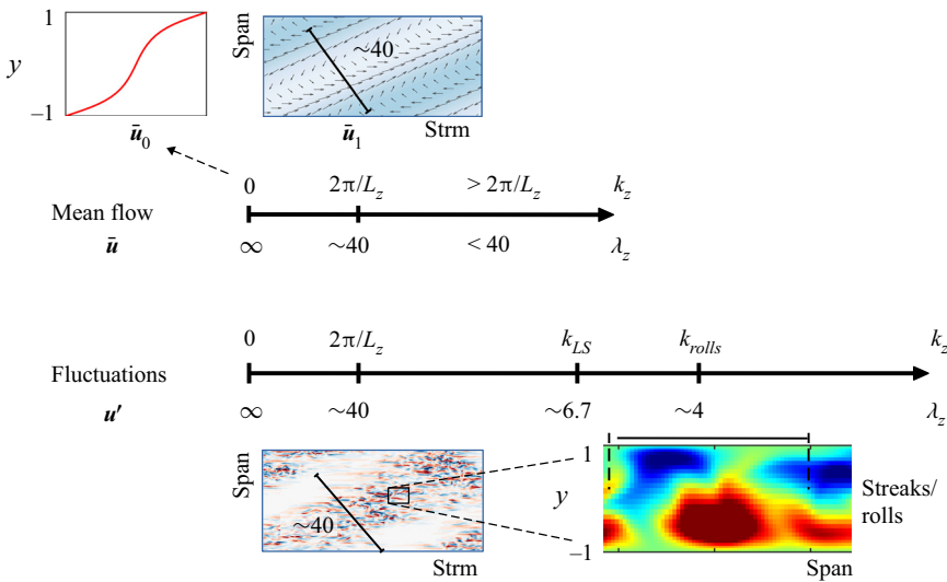
Figure 5. Illustration of the most relevant scales in transitional patterns. The upper part depicts the mean flow: \bar{u}_0 is the uniform ( z -independent) mean shear, illustrated by the mean streamwise velocity profile, while \bar{u}_1 corresponds to scale \lambda_z \sim 40 and is dominated by the flow along the laminar–turbulent interfaces as illustrated in the streamwise–spanwise plane. The lower part depicts the fluctuations: scale \lambda_z \sim 40 is illustrated by the periodic presence and absence of fluctuating cross-flow velocity. The scale k_{LS} is that below which fluctuations receive energy by nonlinear interactions (via \hat{T}_{nl} , (5.3)), and k_{rolls} is the scale of rolls and streaks, illustrated in the spanwise– y plane.
