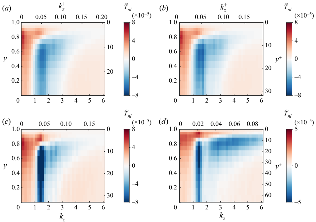
Figure 14. Visualisations of nonlinear transfer \hat{T}_{nl}(y, k_z) for different Re and states. The cross-channel range is from the mid-plane ( y = 0, y^+ = Re_\tau , lower axis) to the wall ( y = 1, y^+ = 0 , upper axis). (a) Pattern, Re = 400 ( Re_\tau = 29.7 ). (b) Pattern, Re = 430 ( Re_\tau = 31.9 ). (c) Uniform, Re = 430 ( Re_\tau = 33.0 ). (d) Uniform, Re = 1000 ( Re_\tau = 66.4 ).
