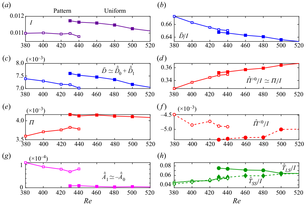
Figure 10. Evolution with Re of various energetic quantities defined throughout the text ((5.6a,b), (5.7a,b) and (5.8)). Open and filled symbols are used for the patterned and uniform states, respectively. In (h), circles and diamonds stand, respectively, for \hat{T}_{LS}/I and \hat{T}_{SS}/I .
