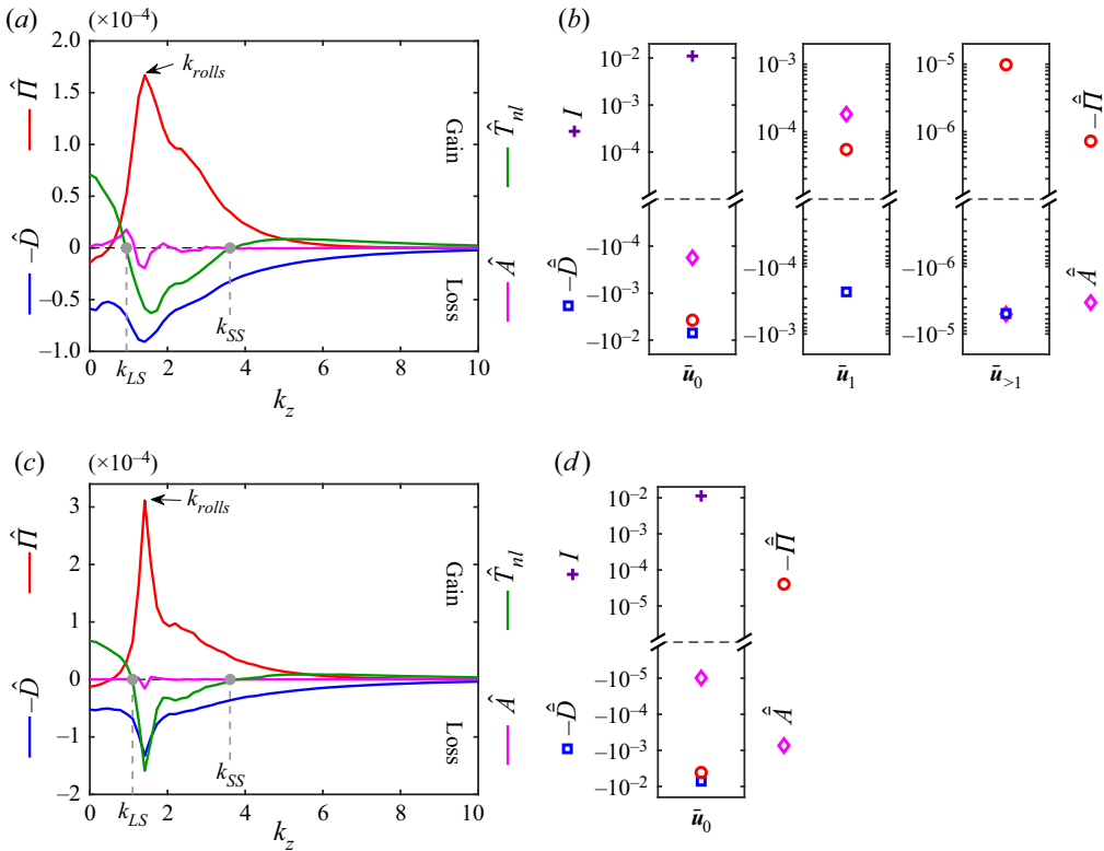
Figure 7. (a) Spectral energy budget (5.3) for a pattern at Re = 400 , integrated over y \in [-1, 1] . Viscous and pressure transfers are not shown as they integrate to 0. The grey circles indicate k_{LS} and k_{SS} , which delimit the spectral region where transfer \hat{T}_{nl} is negative. (b) Spectral energy budget of the mean flow (5.5) for a pattern at Re = 400 , integrated over y \in [-1, 1] , shown for k_z = 0 , k_z = 2\pi/L_z and summed over k_z > 2\pi/L_z . (c,d) Same as (a,b) for a uniform state at Re = 500 . To convey both sign and order of magnitude, (b,d) show \text{sgn}(Q) \log |Q| for each quantity Q .
