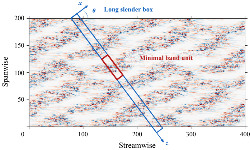
Figure 1. Visualisation of the numerically simulated flow at Re = 360 and our numerical domains. Colours show y velocity at y = 0 (blue -0.2 , white 0 , red 0.2 ) in a domain of size L_{strm} = 400 , L_{span} = 200 . Red and blue boxes show a minimal band unit and a long slender box, respectively.
