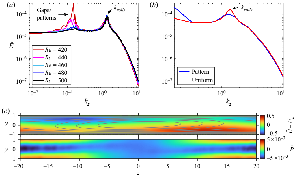
Figure 3. (a) Total energy spectra in a large long slender box L_z = 800 (black line) at y = 0 , for different Re . The spectra are averaged irrespective of the nature of the state (patterned or uniform). (b) Total energy spectra (continuous lines) in a minimal band unit of size L_z = 40 . The spectra are computed individually in the uniform turbulence (red) and patterned states (blue), at Re = 430 . (c) Visualisations of the patterned mean flow in a minimal band unit: colours show the deviation of the along-band velocity from the laminar base flow \bar{U} - U_b (top plot) and the pressure \bar{P} (bottom plot). Streamlines of the mean flow perpendicular to the bands are shown as grey curves. The laminar region is centered at z = 0 .
