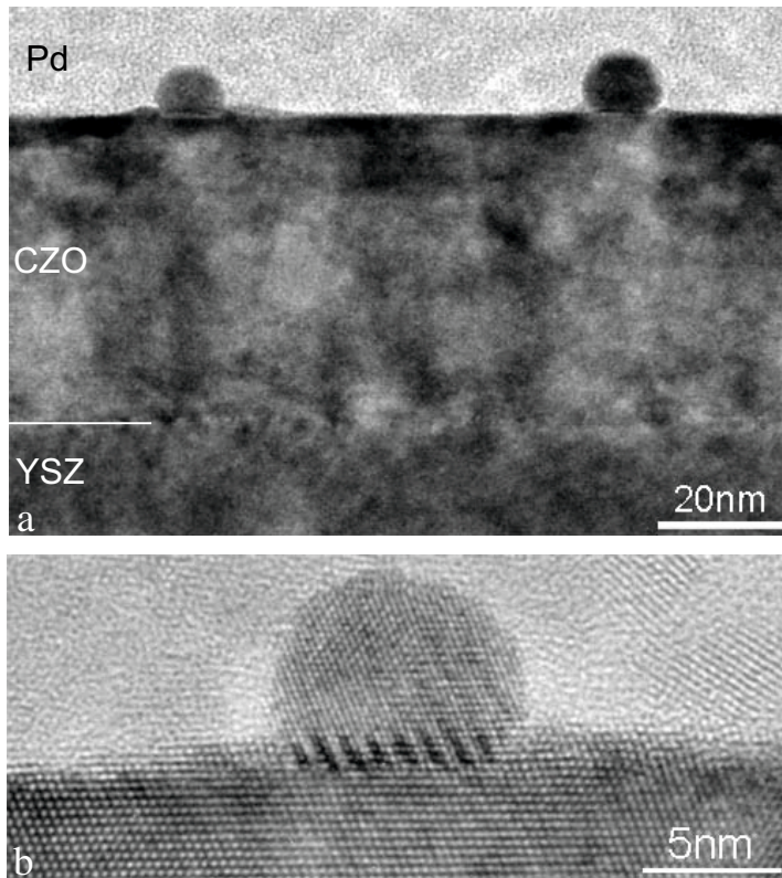
Figure 1. (a) Cross-sectional TEM image of the reduced Pd/CZO model catalyst. (b) HRTEM image shows partial encapsulation of a Pd particle by the CZO support, which indicates a strong metal/oxide interaction.
