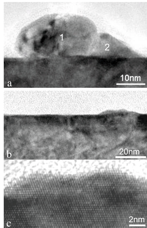
Figure 2. (a) Cross-sectional TEM image of the reoxidized Pd/CZO model catalyst. (b)-(c) Morphology and microstructure of the hillock on CZO surface while Pd particle is missing.
