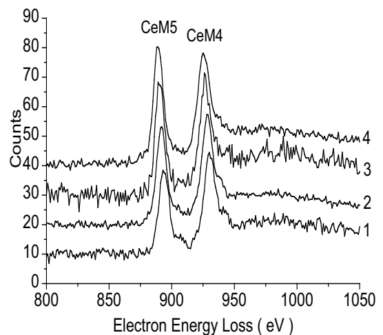
Figure 4. EELS spectra of Ce acquired from CZO/YSZ interface (1, 3) and CZO film surface (2, 4) of the sample before (1, 2) and after reducing (3, 4) treatment.
