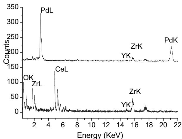
Figure 3. EDS spectra of Pd particle (top) and CZO surface hillock (bottom), which are obtained from area 1 and 2 in Figure 2(a) respectively using 1nm-spot size electron beam.
