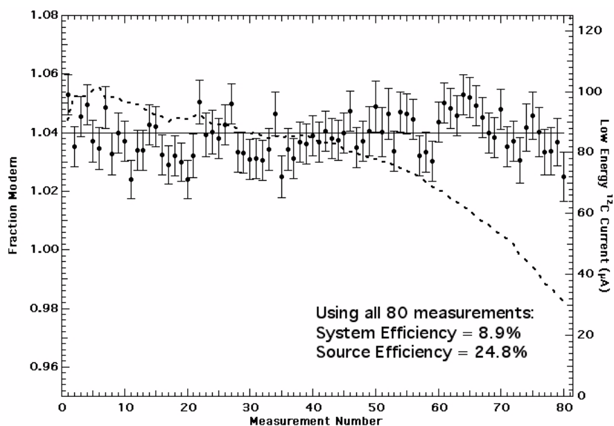
Figure 5 Repeat measurements of a 430- \mu g HOxI. The uncertainty for each point is a combination of statistical and normalization errors. The average low-energy ^{12}\text{C} current (measured on the off-axis Faraday cup) is shown as a dashed line using the right axis. These data demonstrate both the efficiency and stability of the system.
