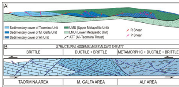
Figure 11. (Colour online) Schematic geometry of the shear zone along the Ali–Taormina Thrust (A) and model of the related structural assemblages in the distinct portion of the shear zone (B).
