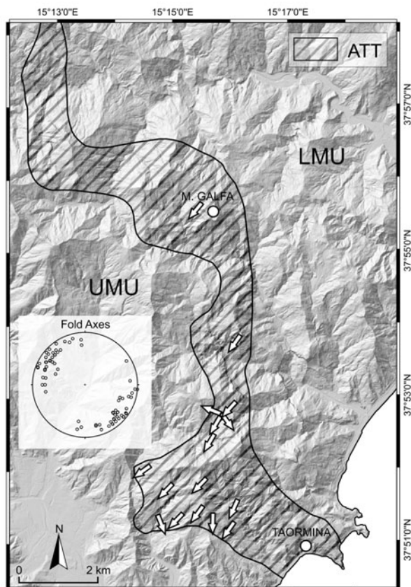
Figure 10. Slip-vectors measured on mesoscale R and P shear planes bounding the carbonate lithons along the Ali–Taormina Thrust in the area from Mount Galfa to Taormina. The stereoplot refers to the mesoscale fold axes measured along this portion of the shear zone.
