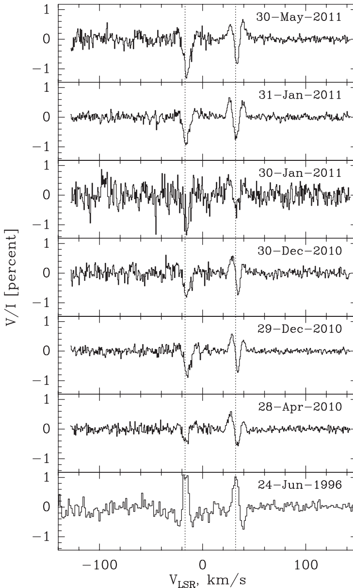
Figure 3. Time sequence of circular polarization spectra obtained with the IRAM 30m telescope. The transition observed is H30 \alpha at 231.9 GHz. Spectra were smoothed to a resolution of 0.4 km s -1 . The vertical dashed lines indicate the peak velocities of the blue- and red-shifted maser spikes.
