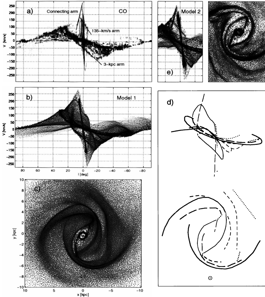
Figure 1. a) Observed CO l - V diagram (Dame et al. 1995), with some relevant features indicated. b-c) Corresponding plot and face-on view for model 1, which provides a fair global qualitative agreement with the data. d) Link between the spiral arms and the l - V features in this model. e-f) Results for model 2, which reproduces almost perfectly the connecting arm. The location of the Sun is indicated by the \odot symbol.
