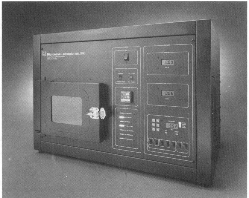
T-4001 Variable Frequency Microwave Furnace* (100-200W CW, 2.4 to 7.5 GHz)
