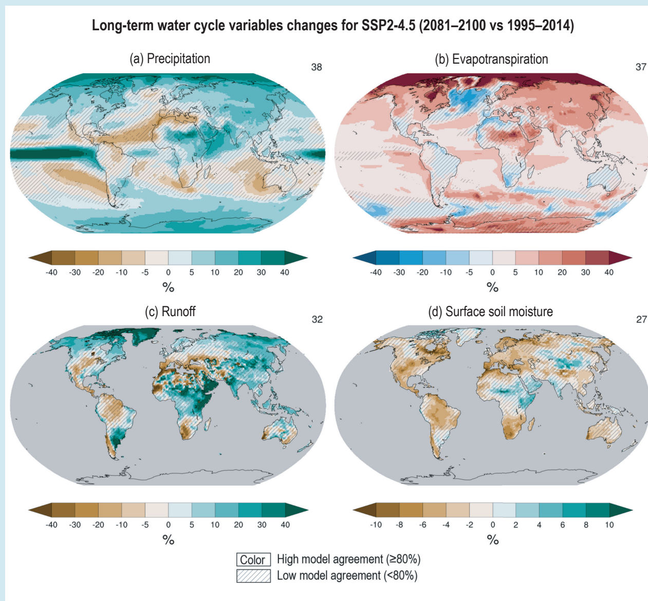
Box TS.6, Figure 1 | Projected water cycle changes. The intent of this figure is to give a geographical overview of changes in multiple components of the global water cycle using an intermediate emissions scenario. Important key message: without drastic reductions in greenhouse gas emissions, human-induced global warming will be associated with widespread changes in all components of the water cycle. Long-term (2081–2100) projected annual mean changes (%) relative to present-day (1995–2014) in the SSP2-4.5 emissions scenario for (a) precipitation, (b) surface evapotranspiration, (c) total runoff and (d) surface soil moisture. Numbers in top right of each panel indicate the number of Coupled Model Intercomparison Project Phase 6 (CMIP6) models used for estimating the ensemble mean. For other scenarios, please refer to relevant figures in Chapter 8. Uncertainty is represented using the simple approach: No overlay indicates regions with high model agreement, where \geq 80\% of models agree on sign of change; diagonal lines indicate regions with low model agreement, where < 80\% of models agree on sign of change. For more information on the simple approach, please refer to the Cross-Chapter Box Atlas.1. [8.4.1; Figures 8.14, 8.17, 8.18, and 8.19]
