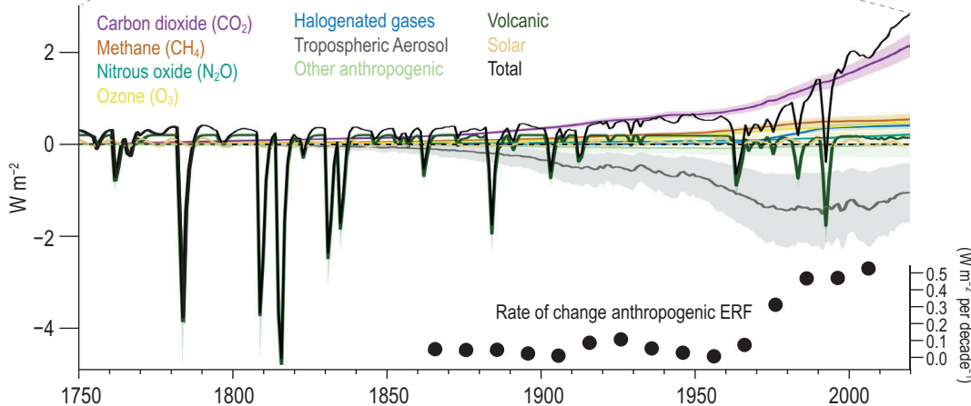
Figure TS.9 | Changes in well-mixed greenhouse gas (WMGHG) concentrations and effective radiative forcing (EFR). The intent of this figure is to show that the changes of the main drivers of climate system over the industrial period are exceptional in a long-term context. (a) Changes in carbon dioxide (CO 2 ) from proxy records over the past 3.5 million years. (b) Changes in all three WMGHGs from ice core records over the Common Era. (c) Directly observed WMGHG changes since the mid-20th century. (d) Evolution of ERF and components since 1750. Further details on data sources and processing are available in the associated FAIR data table. [2.2, Figures 2.3, 2.4 and 2.10]
