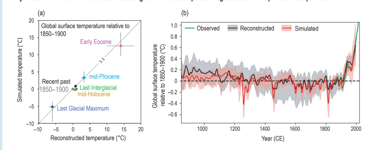
Proxy-based and model-simulated estimates of global surface temperature agree across multiple reference periods
