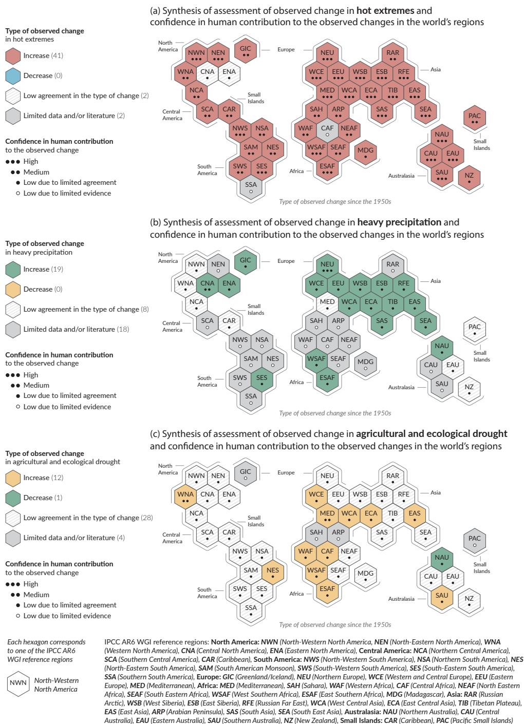
Box TS.10, Figure 1 | Synthesis of assessed observed and attributable regional changes.
