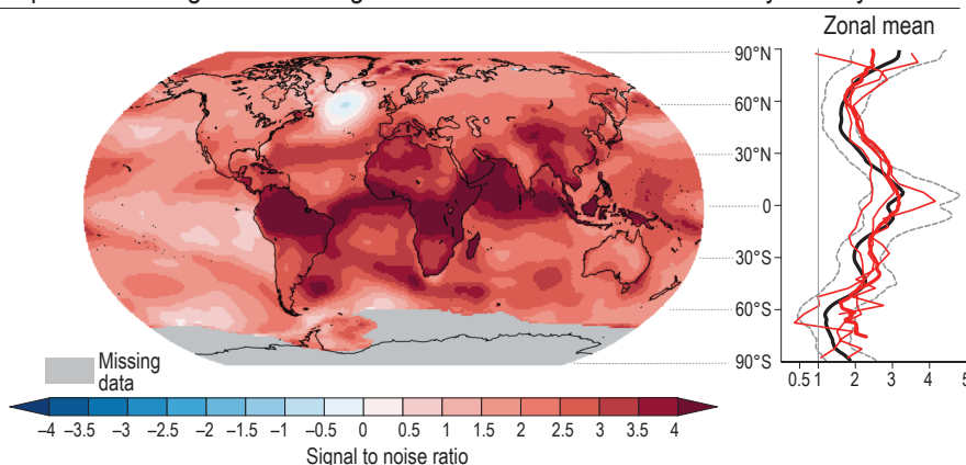
(b) Change in temperature at a global warming level of 1°C relative to the size of year-to-year variations
