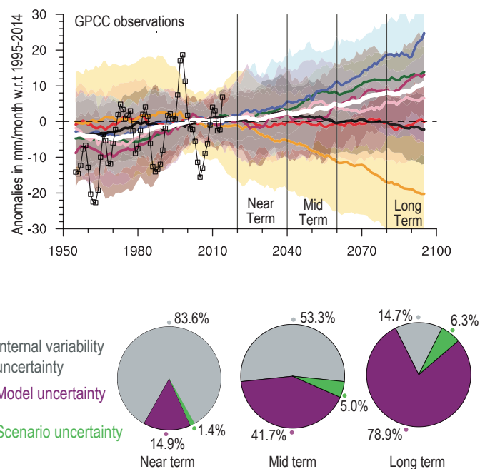
(b) Models simulations/evaluation of SES DJF precipitation over the historical period and 21st century based on 7 large ensembles
