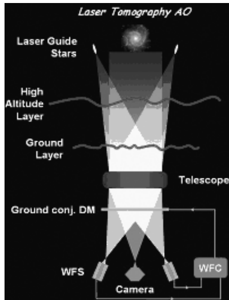
Figure 4. Laser Tomography Adaptive Optics (LTAO) concept
