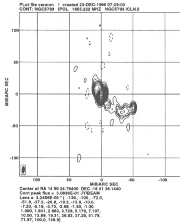
Figure 1. The VLBA continuum map of 1.6 GHz.
