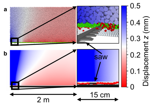
Fig. 7. PST setup of the (a) DEM and (b) MPM modelling while sawing the PST. The colouring in the slab indicates the vertical displacement. The insets (15 cm × 15 cm) show a close-up around the saw. The DEM inset (a) shows slab and weak layer particles in blue and green, respectively. Around the saw particles are clipped and bonding damage in the weak layer is highlighted in red. In the MPM inset (b), the crack (red) started propagating and is already ahead of the snow saw.
