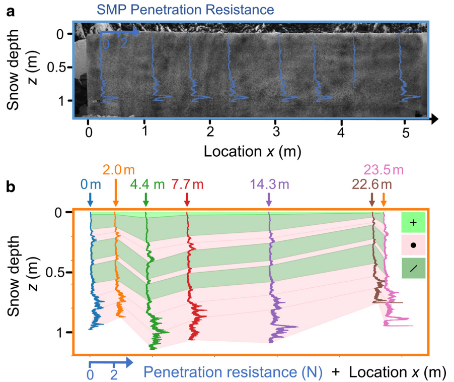
Fig. 3. (a) Penetration resistance measured with the SMP along the PST experiment (blue lines plotted on an image of the speckled side wall of the PST). (b) Penetration resistance measured at each acceleration sensor (indicated by colour as shown in Fig. 4) after triggering the whumpf. The background colours indicate the grain type (top right) of the corresponding layer in the manual profile. Measurements are restricted to the slab to the top of the melt-freeze crust (red layer in Fig. 2b).
