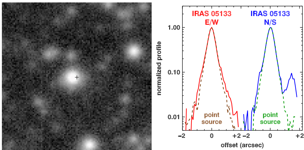
Figure 3. Left: An I -band image of IRAS 05133–6937 from the SOAR Adaptive Module (SAM) covering 10'' \times 10'' . The cross marks the infrared position of the source (Sloan et al. 2016), which is 0.26'' from the center of the I -band source. Right: Profiles of IRAS 05133 showing a low-contrast halo (solid lines) compared to a nominal point source (dashed lines).
