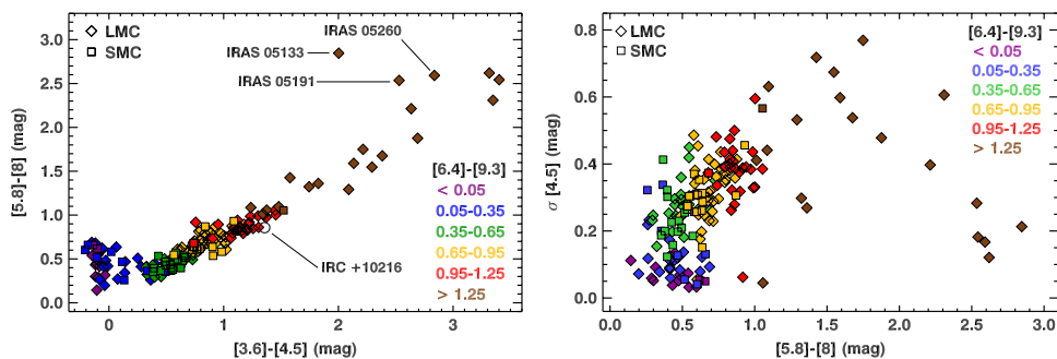
Figure 1. Left: A color-color plot of the IRS sample of Magellanic carbon stars using photometry from Spitzer and WISE . The data are coded by their [6.4]–[9.3] color, which is determined from their spectra and is a good proxy for the amount of dust. See the text for more on the labeled objects. Right: Variability, as measured by the standard deviation of Spitzer and WISE data at 4.5 and 4.6 \mu\text{m} , vs. [5.8]–[8] color. Both plots are adapted from Sloan et al. (2016).
