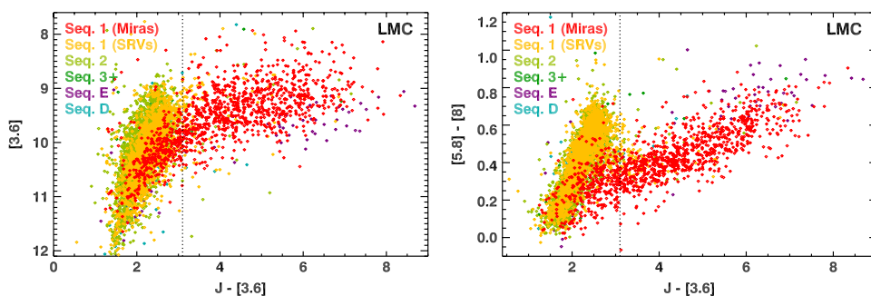
Figure 2. Left: A color-magnitude diagram of carbon stars in the OGLE-III survey (Soszyński et al. 2009), coded by their OGLE-III variability type and pulsation sequence. Right: The same carbon-rich sample in color-color space. The vertical line at J - [3.6] = 3.1 marks the boundary of the extreme AGB as defined by Blum et al. (2006).
