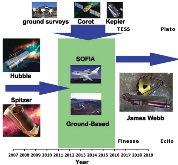
Figure 1. Exoplanet occultation spectrophotometry in the next decade: In the past few years Hubble and Spitzer (left) have been successfully used for spectroscopic characterization of extrasolar planets. As warm Spitzer winds down and Hubble's infrared capabilities are restricted to wavelengths below 1.7 \mu\text{m} , space-based opportunities are limited until JWST (and possibly, if selected FINESSE, EcHo) starts operating. Over the next several years ground-based surveys (such as MEarth, HATNet or KELT) and space-based missions (such as WASP, CoRoT or Kepler and TESS/Plato in the future) (top) will continue to deliver a large number of new targets with interesting opportunities for characterization. The airborne observatory SOFIA will allow follow-up observations of these planets as a testbed for observational strategies and target decision guidance for future observations with (dedicated) space-borne platforms.
