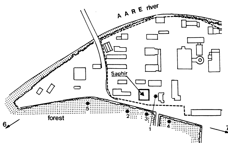
Fig 3. 14 C concentrations around the Saphir research reactor at EIR, given as net values relative to the reference station. Although the release rate is estimated to be below 7 \cdot 10^9 Bq/yr, the measured excess values are quite high. This is because the 14 C activity is released at the roof and the sampling sites are very close to the emission point. The dilution factors are then smaller than at other sites. The samples were also collected at emission height. The decrease of the net activity with distance can be described by a power law.
