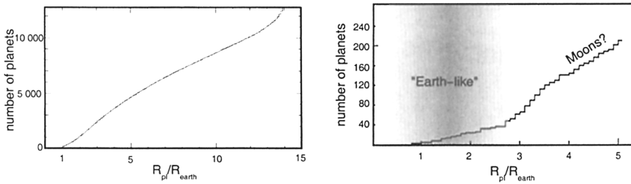
Figure 1. Expected count of detected planets. Left: all planets at any temperature or distance from the central star. Right: planets in the ‘habitable zone’ (250-350K). The field ‘Earth-like’ indicates the size range of planets suitable to support life (solid surface and ability to maintain atmosphere). Moons around larger planets may also indicate life sites.
