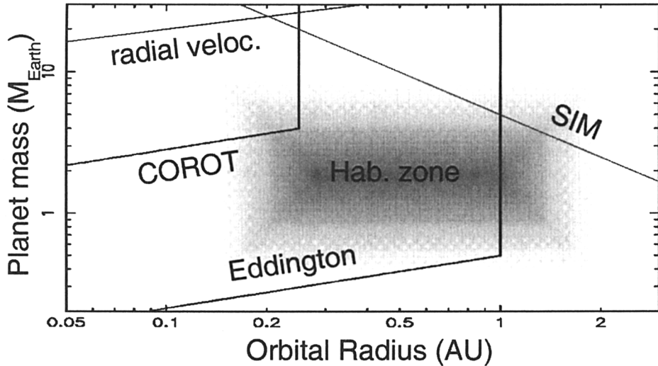
Figure 2. Comparison of planet finding capabilities of several missions. SIM's sensitivity is given for a star at 5pc distance. The limits for ground-based radial velocity searches are for a sensitivity of 1 m/s
