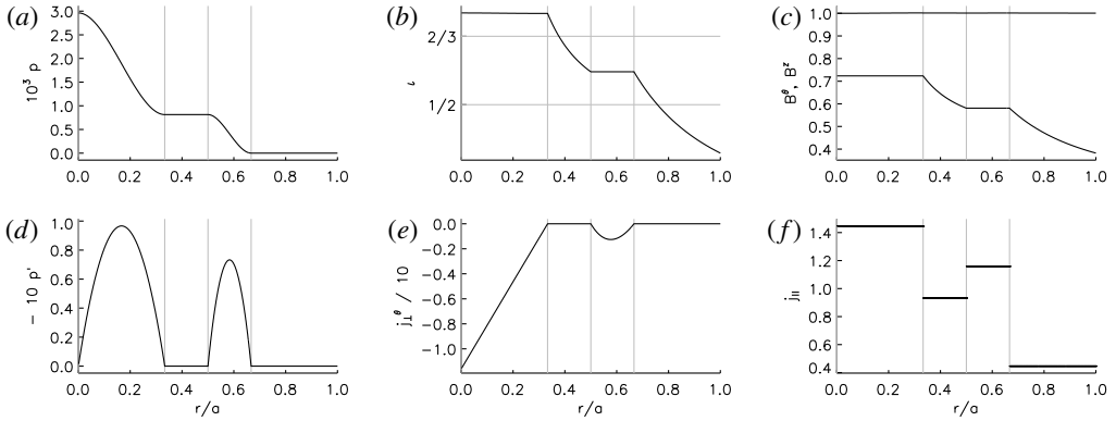
FIGURE 3. An example, in cylindrical geometry, of a mixed ideal–relaxed equilibrium with four regions. (a) The pressure profile. (b) The rotational-transform profile. (c) The ‘toroidal’ and poloidal components of the magnetic field, B^z and B^\theta . (d) The pressure gradient. (e) The poloidal component of the perpendicular current density, j_\perp^\theta . (f) The parallel current density, j_\parallel \equiv \mathbf{j} \cdot \mathbf{B}/B^2 .
