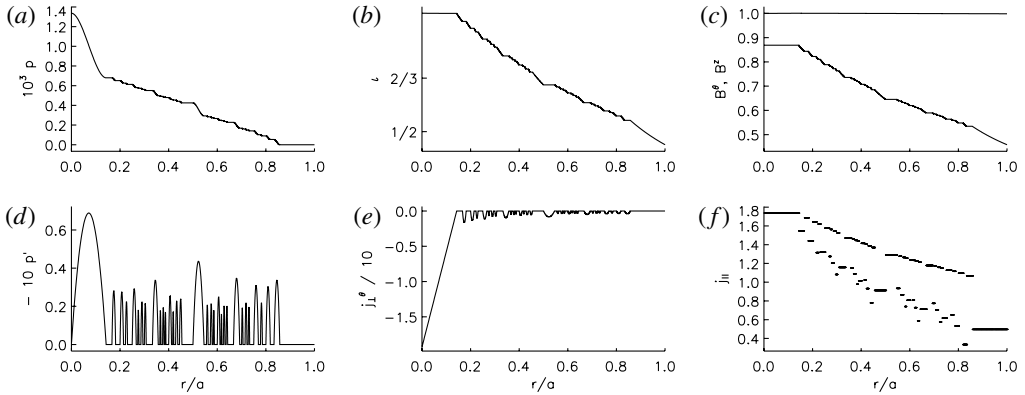
FIGURE 4. Similar to figure 3, but with 64 regions.
