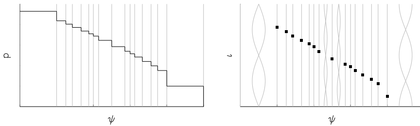
FIGURE 1. Piecewise-constant, discontinuous pressure profile (left), and the discretely defined, strongly irrational rotational-transform profile, with some low-order island chains for illustration.
