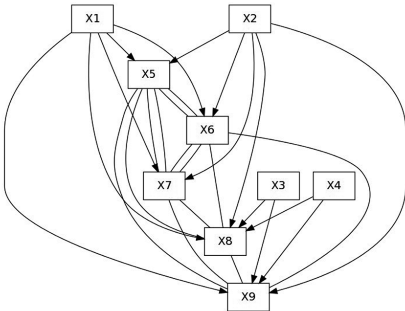
Figure 10. Pattern after running the PC algorithm to find unconditional independence relations.
