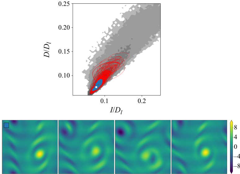
Figure 11. Top: all periodic orbits found via latent Fourier-based recurrent flow analysis at Re = 40 , visualised in terms of their production and dissipation rates (red lines). The laminar dissipation value D_l = Re/(2n^2) . Background grey contours are the turbulent PDF (contour levels spaced logarithmically with a minimum value 10^{-6} ), whereas the blue line identifies the longest UPO found with T = 49.091 , for which we show four snapshots of spanwise vorticity equally spaced every T/5 in the lower four panels of the figure. The starting point for the visualisation of the vorticity is identified with a white square in the production/dissipation plot, whereas contour levels for the vorticity run from -10 \leq \omega \leq 10 .
