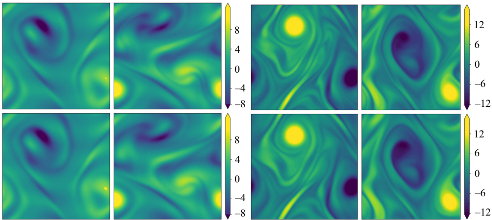
Figure 3. Snapshots of vorticity (top) at Re = 100 (left) and Re = 400 (right). Below is the output of the autoencoder, \omega_{norm}, \mathcal{A}_m(\omega) . The network at Re = 100 has minimum dimension m = 512 , whereas at Re = 400 we use the m = 1024 network. Relative errors (2.5) from left to right are \varepsilon = 0.036 , \varepsilon = 0.065 , \varepsilon = 0.102 and \varepsilon = 0.085 .
