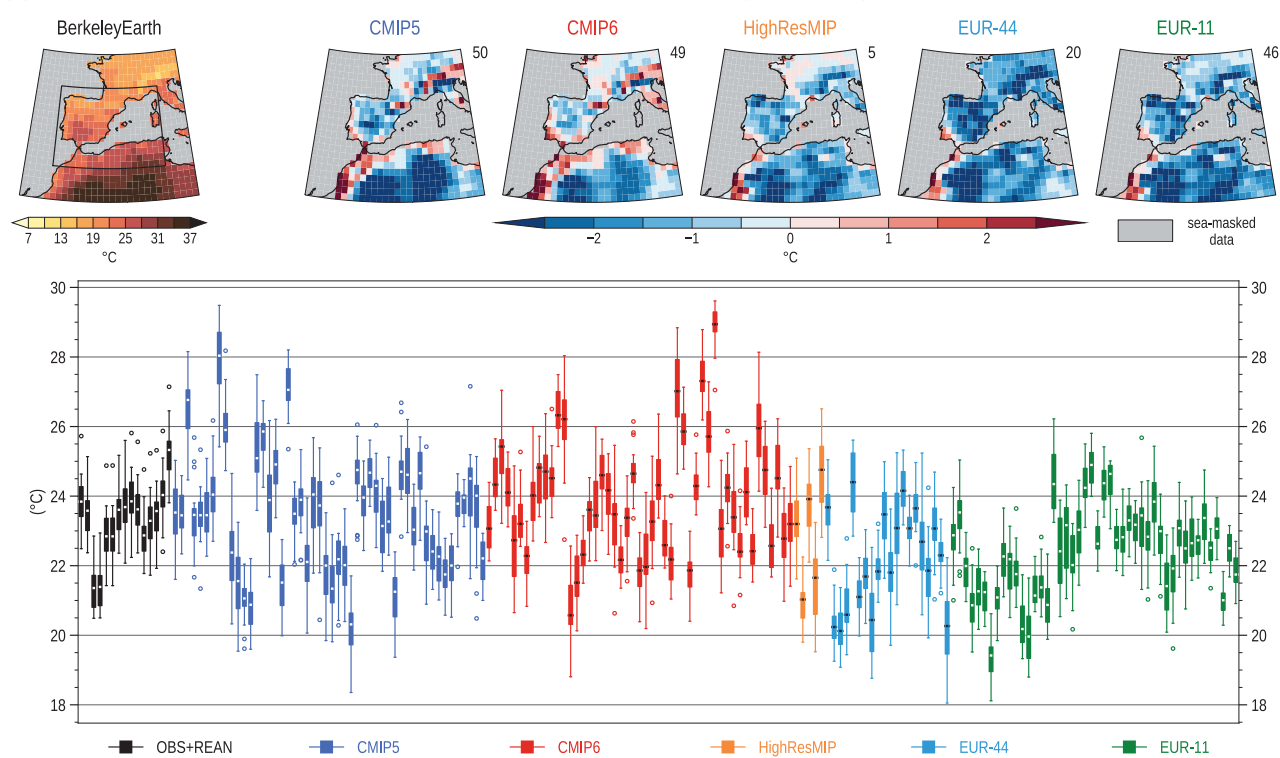
(a) Western Mediterranean June to August mean surface air temperature (1986–2005)
