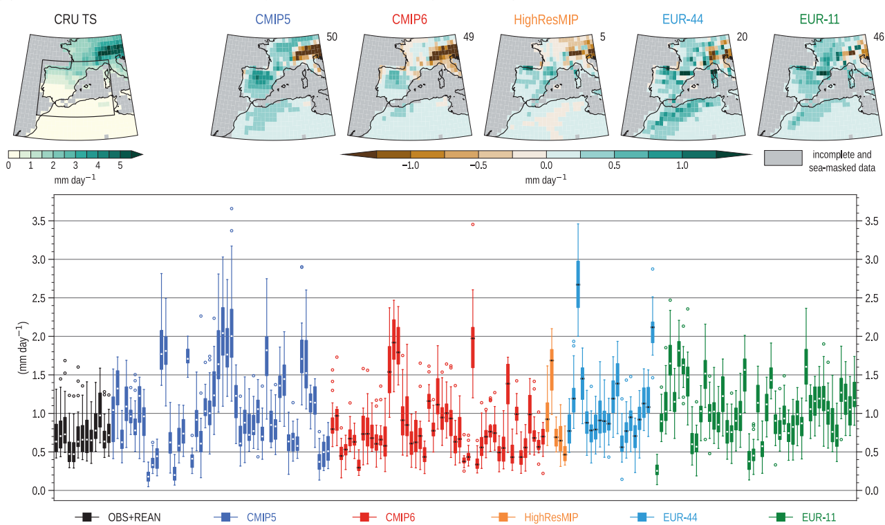
(b) Western Mediterranean June to August mean precipitation (1986–2005)
