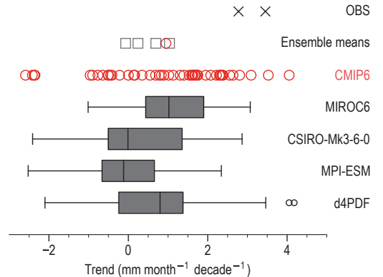
(d) Southeastern South America precipitation trend distribution Trend period (1951-2014)
