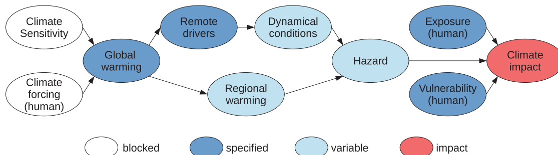
Box 10.2, Figure 1 | Schematic of two types of physical climate storylines with a particular climate impact of concern (red). The storylines are defined by specified elements (dark blue). Variable elements (light blue) are simulated conditional on the specified elements. The white elements are 'blocked' since their state does not need to be known to determine the light blue elements. Other types of storylines could be defined by specifying other elements (e.g., storylines of different climate sensitivities or different representative concentration pathways). (a) Event storyline, where the particular dynamical conditions during the event as well as the regional warming are specified and control the hazard arising from the event. (b) Dynamical storyline, where the global warming level and remote drivers are specified and control the long-term changes in atmospheric dynamics and regional warming. In both storylines, the impact is also conditioned on specified exposure and vulnerability. Figure adapted from Shepherd (2019).
