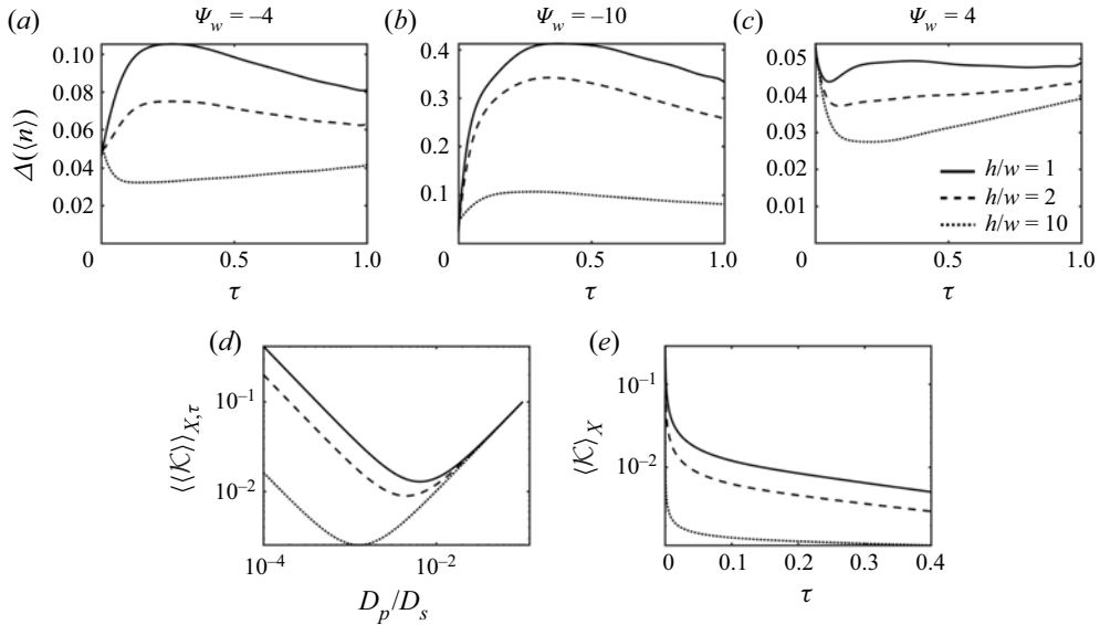
Figure 5. (a)–(c) The full width half-maximum \Delta\langle n \rangle vs time \tau of the colloid distributions \langle n \rangle solved from (4.3) and (A14). The colloid distributions have Gaussian initial distributions and observe no-flux conditions at the pore walls and inlet. The diffusioosmotic velocity and the diffusioosmotic slip are driven by a solute diffusing out of the pore into an infinite reservoir. The initial solute condition is \langle c \rangle(\tau = 0) = 1 and the boundary conditions are \langle c \rangle(X = 0) = 0.1 and no-flux conditions at the pore walls. The full width half-maximum is evaluated for varying pore wall zeta potential ( \Psi_w = -4, -10, 4 ). (d) The non-dimensional modified coefficient of diffusion \mathcal{K} vs non-dimensional particle diffusivity D_p/D_s . The double bracket indicates an average over the length of the pore and the timespan \tau = 0 \rightarrow 0.4 . A minimum is seen in each curve for an intermediate value of particle diffusivity. (e) The non-dimensional modified coefficient of diffusion vs time. The single bracket indicates an average over the length of the pore. Particle diffusivity is chosen to be D_p/D_s = 10^{-3} . A sharp decrease is seen for early times. Each panel demonstrates the effect of increasing cross-sectional aspect ratio h/w to decrease dispersion, indicated by decreasing full width half-maximum (a–c) and decreasing modified coefficient of diffusion (d,e).
