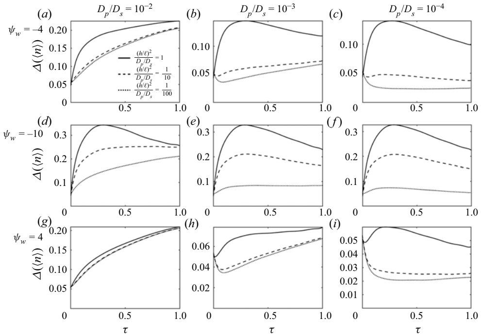
Figure 4. The full width half-maximum \Delta(\langle n \rangle) (see figure 2b) vs time \tau of colloidal particle distributions \langle n \rangle , as obtained by solving (4.3) and (A6). The colloid distributions have Gaussian initial distributions and no-flux conditions at the pore walls and inlet. The diffusiophoretic velocity and the diffusioosmotic wall slip are driven by a solute diffusing out of the pore into an infinite reservoir. The initial solute concentration is \langle c \rangle(\tau = 0) = 1 and the boundary conditions are \langle c \rangle(X = 0) = 0.1 and no-flux conditions at the pore walls. The full width half-maximum is compared for varying particle diffusivity ( D_p/D_s = 10^{-2}, 10^{-3}, 10^{-4} ) and varying pore wall zeta potential ( \Psi_w = -4, -10, 4 ). Furthermore, each panel shows the full width half-maximum for three values of the ratio (h/\ell)^2/(D_p/D_s) : 1, 1/10 and 1/100.
